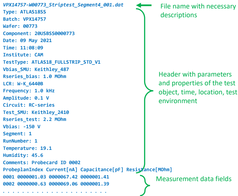
Figure 5: An example of the local data format for one of the QC tests, called Full Strip Test.
