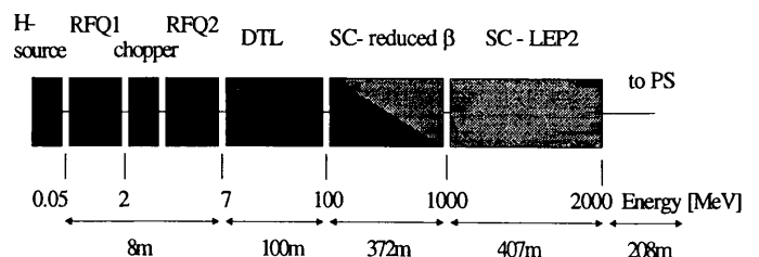
Figure 1: Schematic layout of the Linac.
