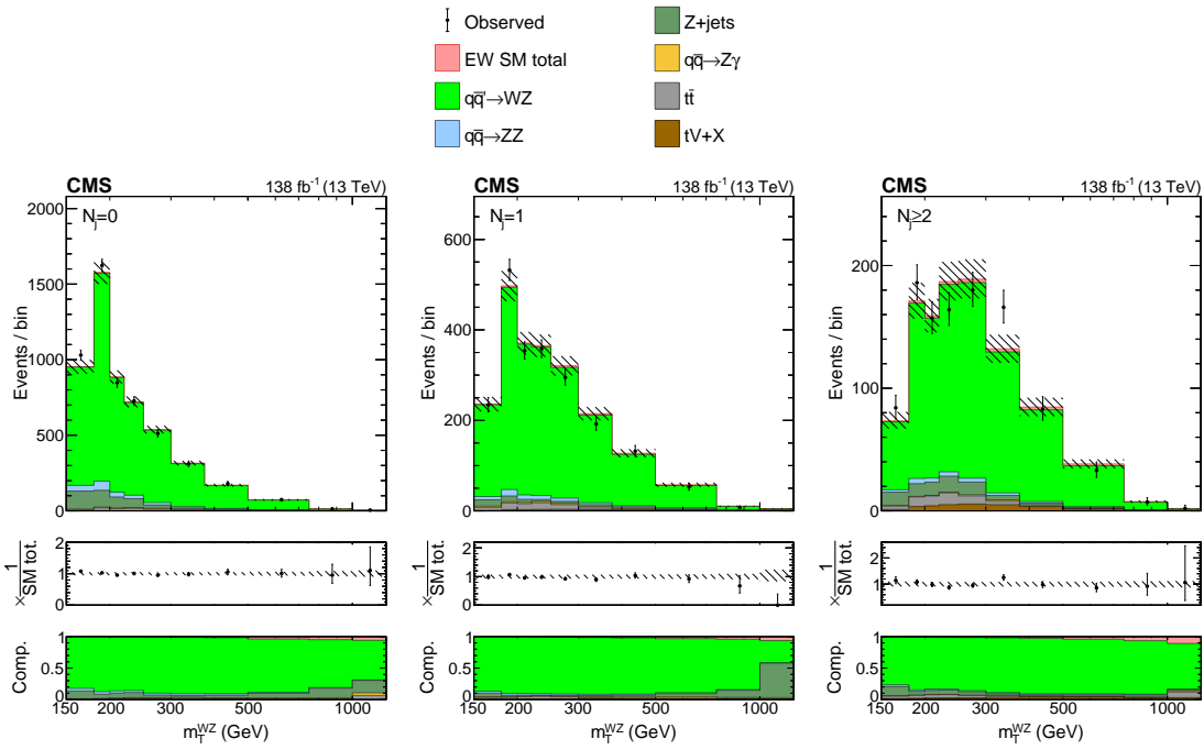
Extended Data Figure 7: Distributions of m_T^{WZ} in different N_j categories of the WZ control region. The postfit distributions of the transverse WZ invariant mass are displayed for the N_j = 0 , N_j = 1 , and N_j \geq 2 jet multiplicity categories of the WZ \rightarrow 3\ell 1\nu control region from left to right. Postfit refers to a combined 2\ell 2\nu + 4\ell fit, together with this control region, assuming SM H boson parameters. The stacked histogram is shown with the hashed band as the total postfit uncertainty at 68% CL. The color legend is given above the plots, with the different contributions referring to the WZ (light green), ZZ (blue), Z+jets (dark green), Z\gamma (yellow), t\bar{t} (gray), and tV+X (brown, with X being any other particle) production processes, as well as the small EW ZZ production component (dark pink). The black points with error bars as uncertainties at 68% CL show the observed data. The middle panels along the vertical show the ratio of the data to the total prediction, and the lower panels show the predicted relative contributions of each process. The rightmost bins contain the overflow.
