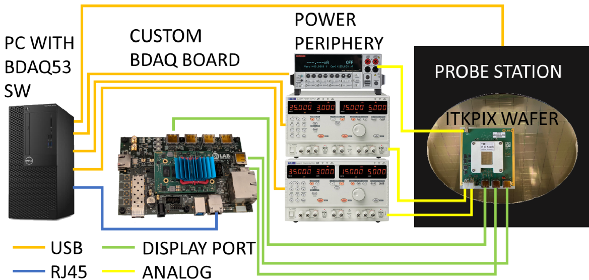
Figure 2: ITkPix wafer probing setup.
