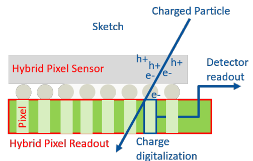
Figure 1: Charge produced by an ionizing particle is guided through a bump bond to the ITkPix readout chip.
