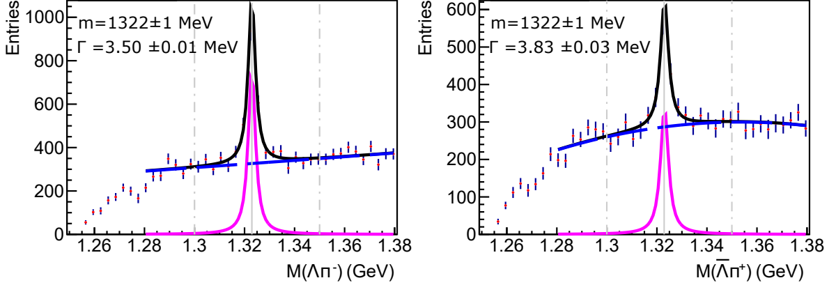
Figure 2: (Color online) Left : The \Lambda\pi^- invariant mass spectrum of \Xi^- candidates for rapidity y between -0.25 and 0.25 and transverse momentum \mathbf{p}_T from 0.4 to 0.6 GeV/c. Magenta line represents the fitted Lorentzian function and blue one shows the fitted background, black line represents their sum. The vertical solid gray line shows the nominal PDG \Xi mass, dashed lines show the integration range used. Right : Analogous \Lambda\pi^+ invariant mass spectrum of \Xi^+ candidates.
