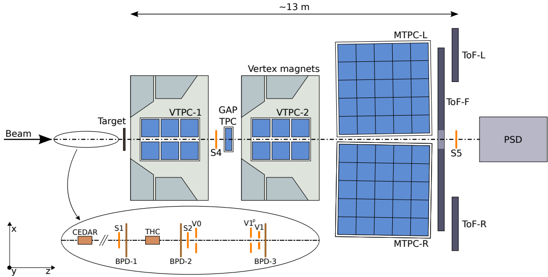
Figure 1: (Color online) Schematic layout of the NA61/SHINE experiment at the CERN SPS (horizontal cut, not to scale). The orientation of the NA61/SHINE coordinate system is shown on the picture. The nominal beam direction is along the z axis. The magnetic field bends charged particle trajectories in the x - z plane. The electron drift direction in the TPCs is along the y (vertical) axis.
