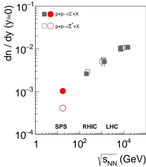
Figure 6: (Color online) Mid-rapidity densities ( dn/dy ) of \Xi^- (full symbols) and \Xi^+ (open symbols) measured in inelastic p+p interactions as a function of centre-of-mass energy \sqrt{s_{NN}} . The systematic and statistical uncertainties are smaller than the symbol size. The data are compared to results from STAR at the BNL RHIC measured at \sqrt{s_{NN}} = 200 GeV [17], from ALICE at CERN LHC measured at \sqrt{s_{NN}} = 0.9, 7 and 13 TeV [18–20] and from CMS at the CERN LHC measured at \sqrt{s_{NN}} = 0.9 and 7 TeV [21].
