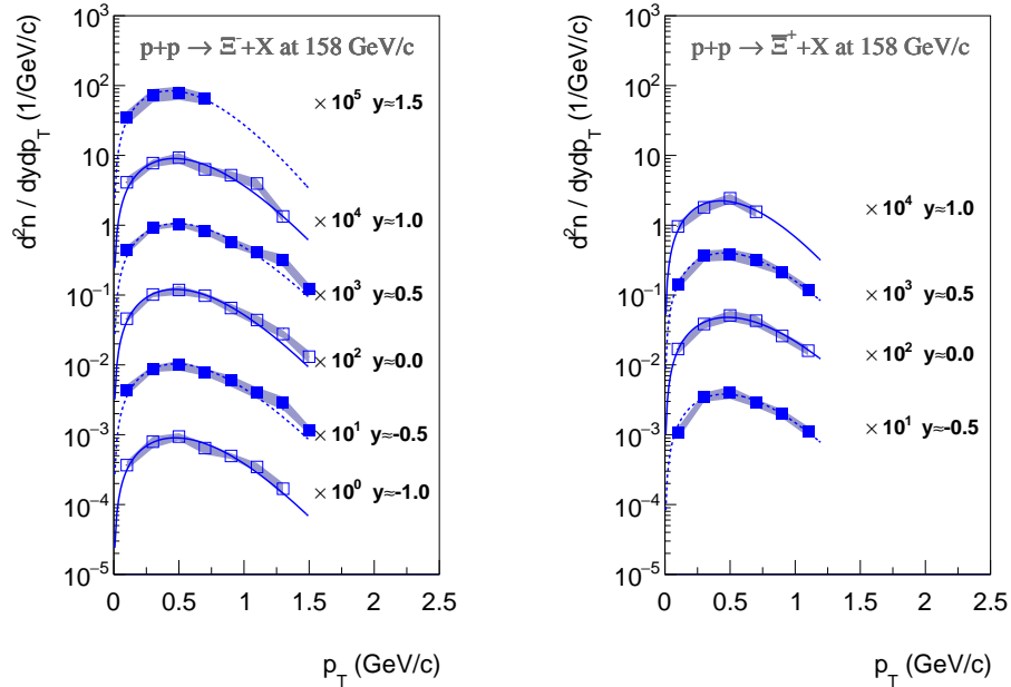
Figure 4: (Color online) Transverse momentum spectra in rapidity slices of \Xi^- (left) and \Xi^+ (right) produced in inelastic p+p interactions at 158 GeV/c. Rapidity values given in the legends correspond to the middle of the corresponding interval. Statistical uncertainties are smaller than the marker size, shaded bands show systematic uncertainties. Spectra are scaled by the given factors for better separation.
