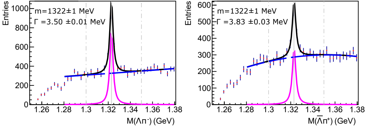
Figure 2: (Color online) Left : The \Lambda\pi^- invariant mass spectrum of \Xi^- candidates for rapidity y between -0.25 and 0.25 and transverse momentum p_T from 0.4 to 0.6 GeV/ c . Magenta line represents the fitted Lorentzian function and blue one shows the fitted background, black line represents their sum. The vertical solid gray line shows the nominal PDG \Xi mass, dashed lines show the integration range used. Right : Analogous \Lambda\pi^+ invariant mass spectrum of \Xi^+ candidates.
