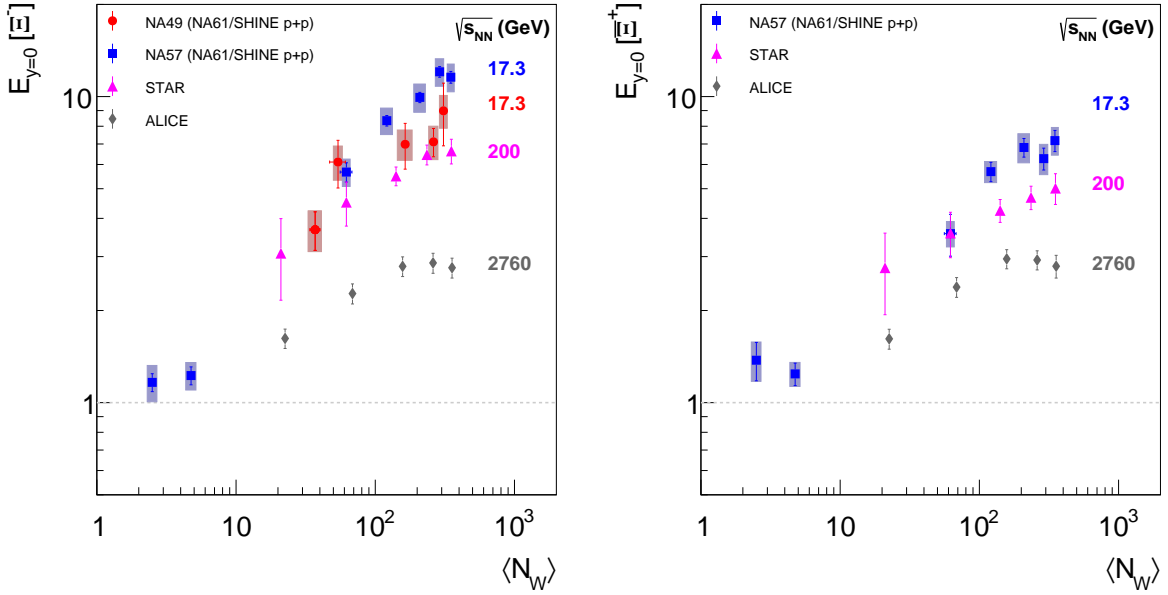
Figure 7: (Color online) The strangeness enhancement E at the mid-rapidity as a function of average number of wounded nucleons \langle N_W \rangle calculated as a ratio of rapidity density for \Xi^- production ( left ) and \bar{\Xi}^+ production ( right ) in nucleus-nucleus interactions per \langle N_W \rangle divided by the corresponding value for p+p interactions (see Eq. 4). Red circles – NA49 Pb+Pb at 158A GeV [27], blue squares – NA57 p+Be , p+Pb and Pb-Pb at the same center-of-mass energy \sqrt{s_{NN}} = 17.3 GeV [25], magenta triangles – STAR Au+Au at \sqrt{s_{NN}} = 200 GeV [28], gray diamonds – ALICE Pb+Pb at \sqrt{s_{NN}} = 2.76 TeV [29]. The systematic errors are represented by shaded boxes.
