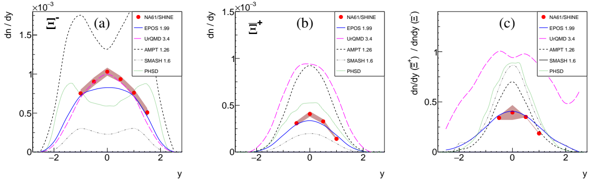
Figure 9: (Color online) Rapidity spectra of \Xi^- (left), \Xi^+ (middle) and \Xi^+/\Xi^- ratio (right) measured in inelastic p+p interactions at 158 GeV/c. Shaded bands show systematic uncertainties. UrQMD 3.4 [34, 35], EPOS 1.99 [33], AMPT 1.26 [36–38], SMASH 1.6 [39–41] and PHSD [42, 43] predictions are shown as magenta, blue, black, gray and green lines, respectively.
