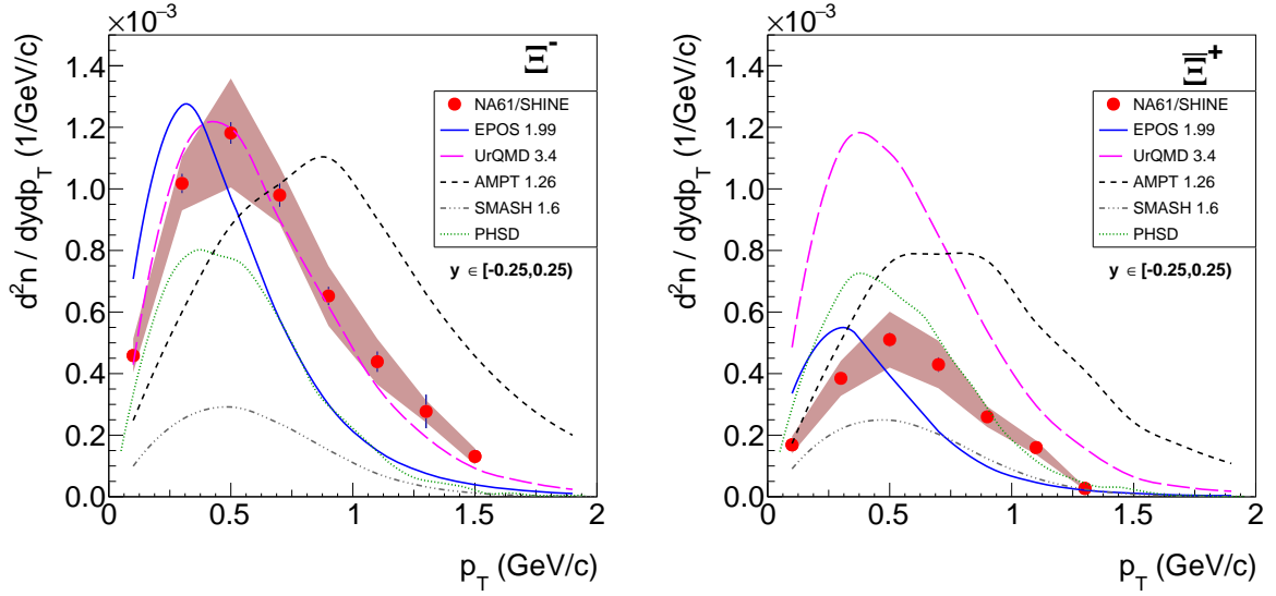
Figure 8: (Color online) Transverse momentum spectra at mid-rapidity of \Xi^- (left) and \Xi^+ (right) produced in inelastic p+p interactions at 158 GeV/c. Rapidity range is included in the legends. Shaded bands show systematic uncertainties. UrQMD 3.4 [34, 35], EPOS 1.99 [33], AMPT 1.26 [36–38], SMASH 1.6 [39–41] and PHSD [42, 43] predictions are shown as magenta, blue, black, gray and green lines, respectively.
