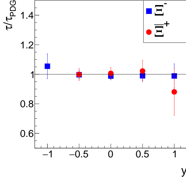
Figure 3: (Color online) Measured lifetime ratio \tau/\tau_{PDG} for \Xi^- (blue squares) and \Xi^+ (red circles) as a function of center of mass rapidity. Only statistical uncertainties are shown.
