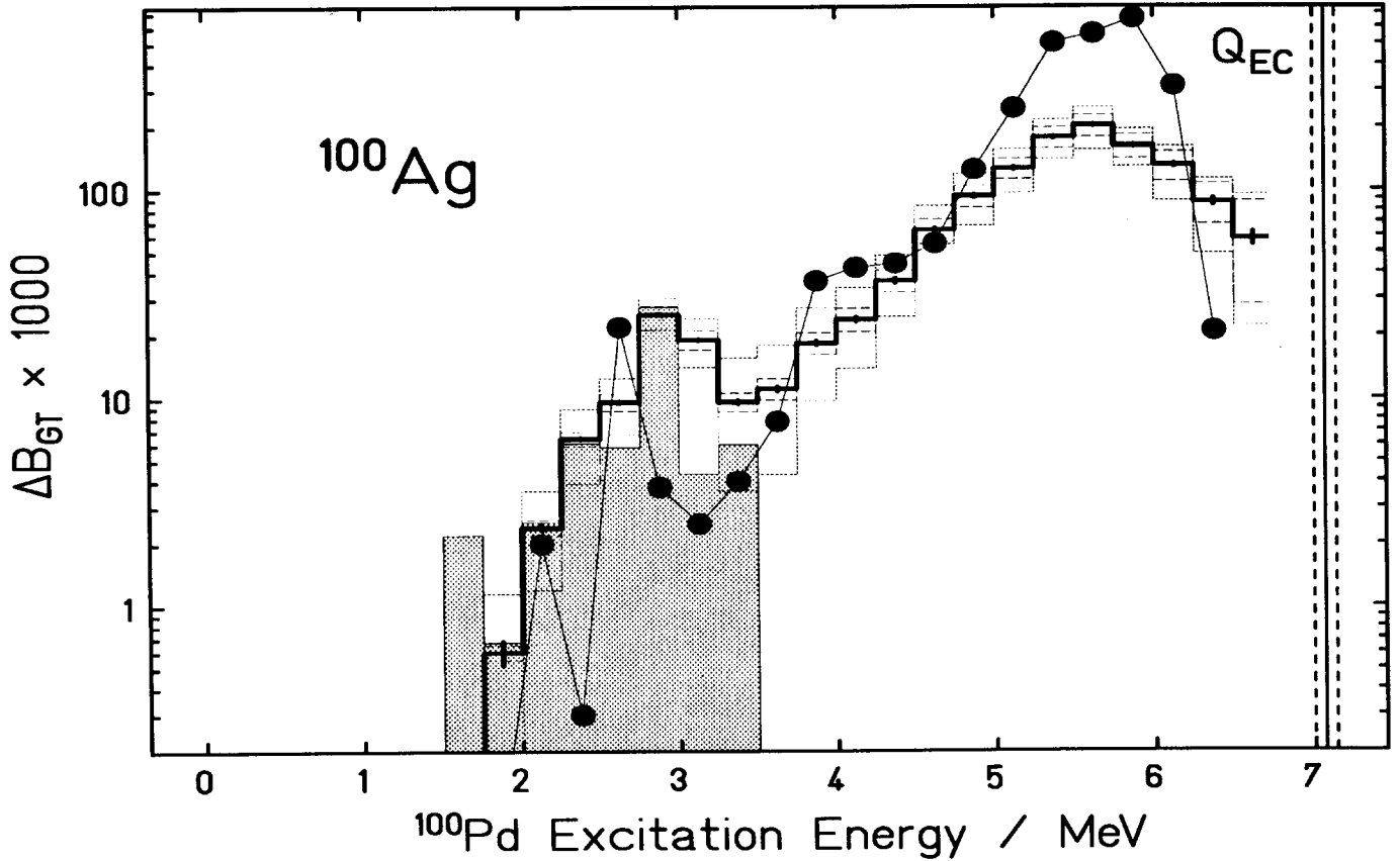
Figure 1: GT-strength distribution for the decay of ^{100}\text{Ag} summed up for intervals of 250 keV (solid histogram). The vertical bars denote the statistical uncertainties for each data point. The total systematical error, displayed by the dotted histograms consists of a contribution from the uncertainty in the Q_{EC} -value (dashed histogram) and from uncertainties in the deexcitation pattern of ^{100}\text{Pd} . The dashed histogram shows the results from a high-resolution study [9] and the smooth line connecting full circles represents the calculated GT-strength of the ^{98}\text{Ag} decay from [5]. The experimental Q_{EC} value of ^{100}\text{Ag} is indicated by a vertical line with the uncertainty given as dashed lines.
