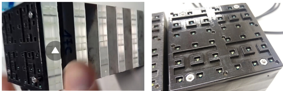
Fig. 6. PLAS reference calorimeter. Left: the absorber-scintillator stack before wrapping with black tape. Right: a detail on the 3D-printed mask used to interface the WLS fibers and the SiPM mounted on the PCB.
