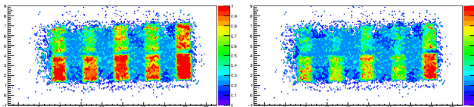
Fig. 14. Lateral efficiency maps at different thresholds of 30 (left) and 35 (right) ADC counts for the upstream module as an example (color version online).
