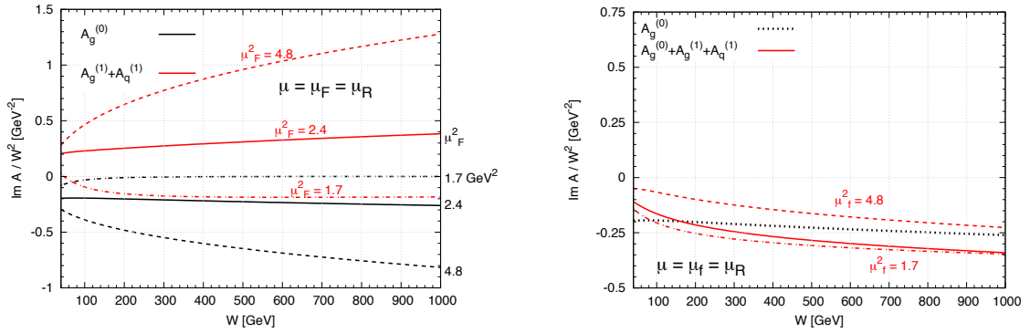
Figure 2: \overline{\text{MS}} scale variations of \text{Im } A/W^2 vs. W at LO and NLO generated using CTEQ6.6 partons at \mu_F^2 = \mu_R^2 = Q_0^2, m_c^2, 2m_c^2 (left panel). The corresponding plot with now the scale fixing and Q_0 cut implemented, with variations now made w.r.t \mu_f = \mu_R and \mu_F^2 = m_c^2 = 2.4 \text{ GeV}^2 fixed (right panel). Q_0 = 1.3 \text{ GeV} is the starting PDF scale for CTEQ6.6.
