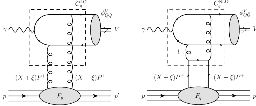
Figure 1: The LO gluon initiated (left panel) and NLO quark initiated (right panel) J/\psi production diagrams. Here the F_i are the GPDs, the dashed boxed encloses the perturbatively calculable five leg coefficient function and \phi_{Q\bar{Q}}^V describes the formation of the J/\psi .
