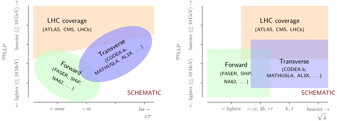
FIG. 4: Schematic summary of reach and coverage of various current, planned or proposed experiments in the LLP mass, lifetime, and \sqrt{\hat{s}} space.
