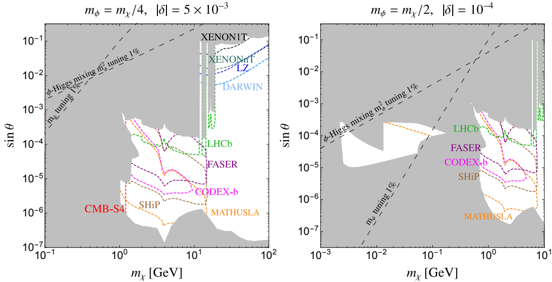
FIG. 20: Projected sensitivity to the coannihilation dark matter benchmark, reproduced from Ref. [133] with permission of the authors. The projections are effectively the same as those in Fig. 9a. In every point of the plot, \Delta is fixed to reproduce the observed relic density. Left: The remaining parameters are set as y = e^{i\pi/4} , m_\phi = m_\chi/4 and \delta = 5 \times 10^{-3} e^{i\pi/4} , with \delta \equiv \delta m/m_\chi . Right: The remaining parameters are set instead as y = e^{i\pi/4} , m_\phi = m_\chi/2 and \delta = 10^{-4} e^{i\pi/4} . MATHUSLA sensitivity is shown for the 200m \times 200m configuration, while FASER sensitivity is shown for the 1m radius configuration, now referred to as FASER2.
