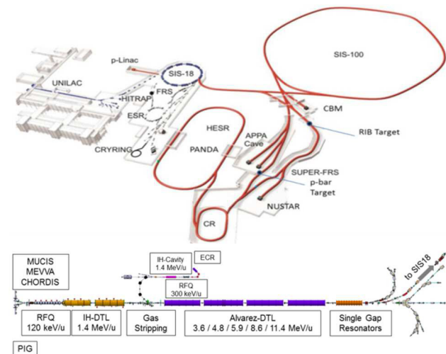
Figure 1: GSI / FAIR facility and the UNILAC injector.
