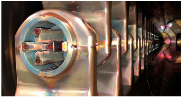
Figure 2: Picture inside the HSI RFQ with the electrodes, carrier rings, stems and one of the tuners.
