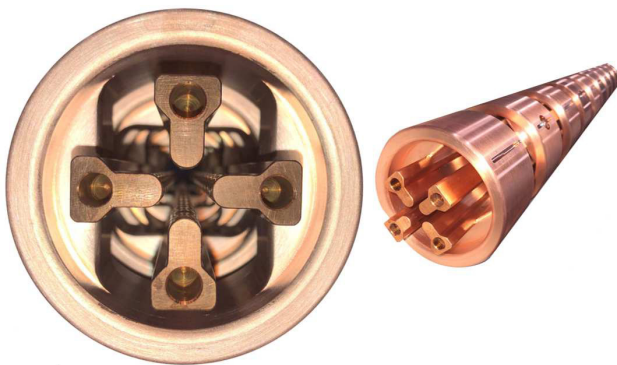
Figure 5: Electrode “basket” of the re-produced electrodes for the second tank section.
