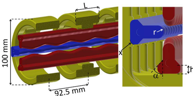
Figure 6: Electrodes and carrier rings of the simulation model with the changeable parameters for the RF simulations.
