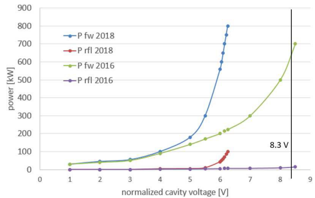
Figure 3: Forward and reflected power 2016 and 2018 as functions of the normalized cavity voltage.
