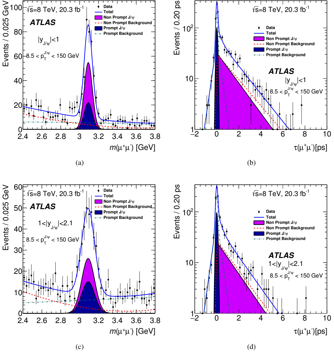
Figure 1: (a) J/\psi candidate mass and (b) pseudo proper decay time for the rapidity range |y_{J/\psi}| < 1 and p_T range 8.5 < p_T^{J/\psi} < 150 GeV; (c) J/\psi candidate mass and (d) pseudo proper decay time for the rapidity range 1 < |y_{J/\psi}| < 2.1 and p_T range 8.5 < p_T^{J/\psi} < 150 GeV.
