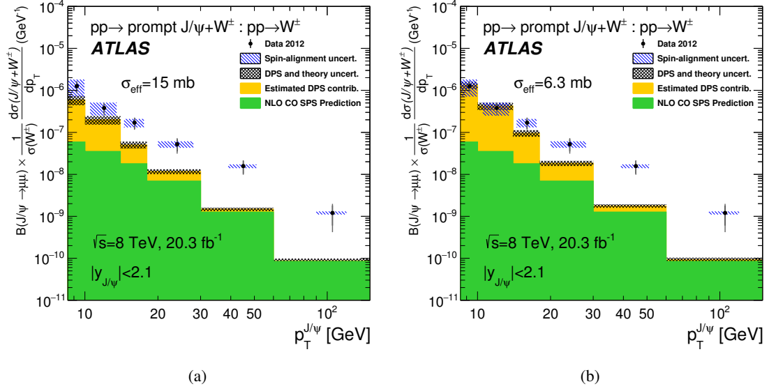
Figure 3: The inclusive (SPS+DPS) differential cross-section ratio measurements and theory predictions presented in six p_T^{J/\psi} regions for |y_{J/\psi}| < 2.1 . NLO colour-octet SPS predictions are shown, with LDMEs extracted from the differential cross-section and spin alignment of prompt J/\psi mesons at the Tevatron [13, 14]. The DPS contribution is estimated using (a) \sigma_{\text{eff}} = 15^{+5.8}_{-4.2} mb and (b) \sigma_{\text{eff}} = 6.3 \pm 1.9 mb and the method discussed in the text. The data points are identical in the two plots.
