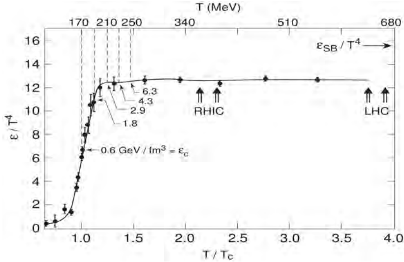
Figure 2.5: Energy density \varepsilon/T^4 vs T/T_c for QCD with 3 light quark flavors [Han01, Kar00].
