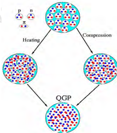
Figure 2.3: Schematic showing QGP formation according to the Bag Model [Cho74].
