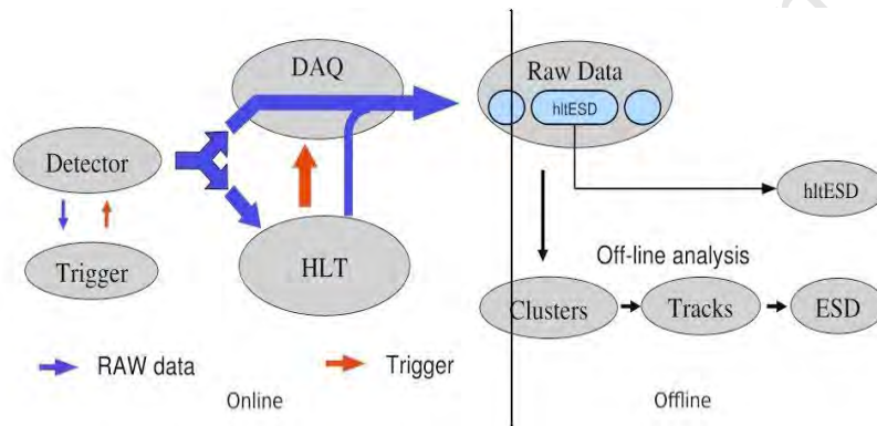
Figure 3.13: Raw data flow scheme showing the relationship between Online and Offline [Ric09].
