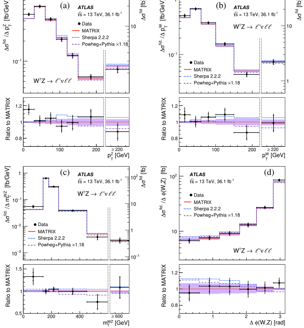
Figure 4: The measured W^\pm Z differential cross section in the fiducial phase space as a function of (a) p_T^Z , (b) p_T^W , (c) m_T^{WZ} and (d) \Delta\phi(W,Z) . The inner and outer error bars on the data points represent the statistical and total uncertainties, respectively. The measurements are compared with the NNLO prediction from MATRIX (red line, see text for details). The violet band shows how the QCD scale uncertainties affect the NNLO predictions. The predictions from the POWHEG+PYTHIA and SHERPA MC generators are also indicated by dotted-dashed and dashed lines, respectively. In (a), (b) and (c), the right vertical axis refers to the last cross-section point, separated from the others by vertical dashed lines, as this last bin is integrated up to the maximum value reached in the phase space and the cross section is not divided by the bin width.
