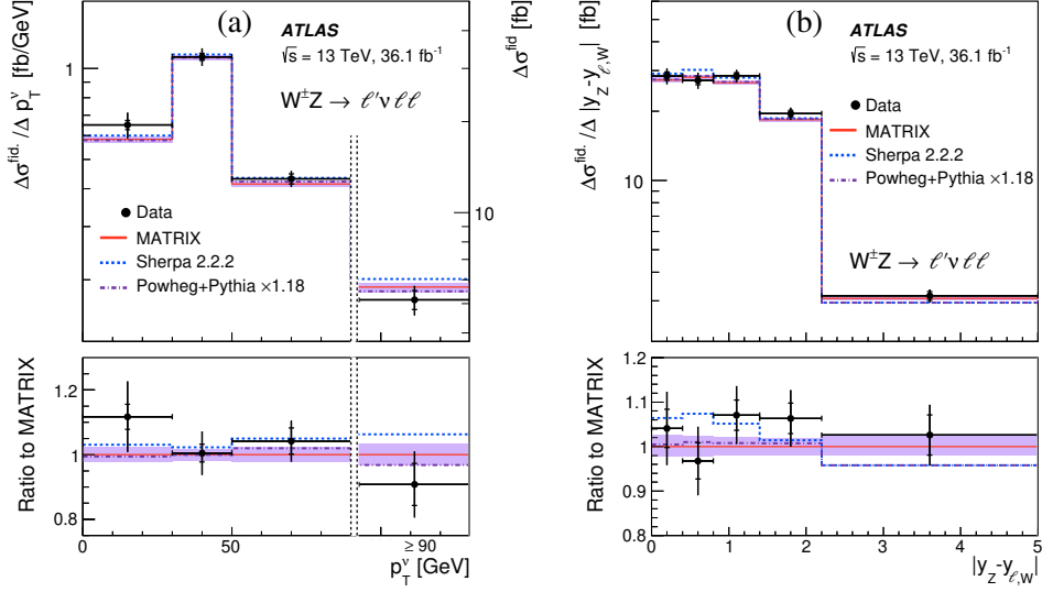
Figure 5: The measured W^\pm Z differential cross section in the fiducial phase space as a function of (a) p_T^Y and (b) |y_Z - y_{\ell,W}| . The inner and outer error bars on the data points represent the statistical and total uncertainties, respectively. The measurements are compared with the NNLO prediction from MATRIX (red line, see text for details). The violet band shows how the QCD scale uncertainties affect the NNLO predictions. The predictions from the POWHEG+PYTHIA and SHERPA MC generators are also indicated by dotted-dashed and dashed lines, respectively. In (a), the right vertical axis refers to the last cross-section point, separated from the others by vertical dashed lines, as this last bin is integrated up to the maximum value reached in the phase space and the cross section is not divided by the bin width.
