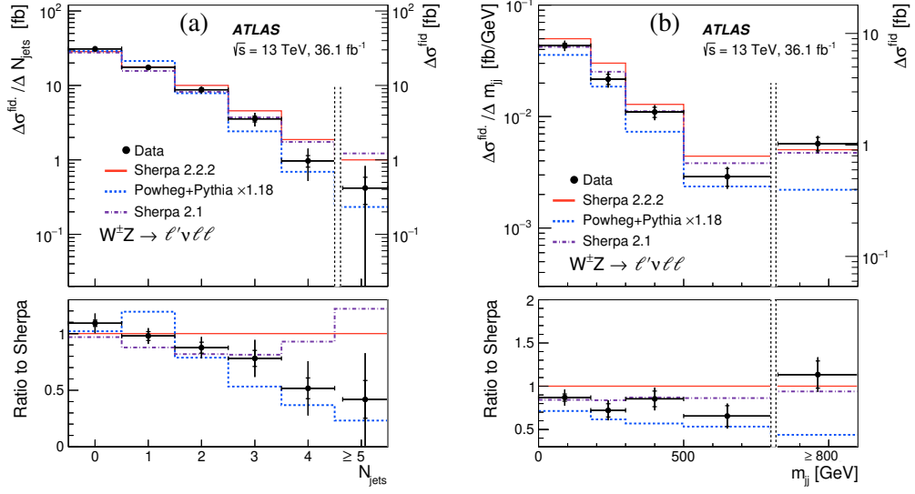
Figure 6: The measured W^\pm Z differential cross section in the fiducial phase space as a function of the exclusive multiplicity of jets with p_T > 25 GeV (a) and of the invariant mass of the two leading jets with p_T > 25 GeV (b). The inner and outer error bars on the data points represent the statistical and total uncertainties, respectively. The measurements are compared with the predictions from SHERPA 2.2.2 (red line), POWHEG+PYTHIA (dashed blue line) and SHERPA 2.1 (dotted-dashed violet line). The right vertical axis refers to the last cross-section point, separated from the others by vertical dashed lines, as this last bin is integrated up to the maximum value reached in the phase space and the cross section is not divided by the bin width.
