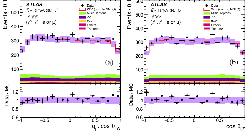
Figure 9: The detector-level distributions for the sum of all channels of the variables (a) q_\ell \cdot \cos \theta_{\ell,W} and (b) \cos \theta_{\ell,Z} . The points correspond to the data with the error bars representing the statistical uncertainties, and the histograms correspond to the predictions of the different SM processes. The sum of the background processes with misidentified leptons is labelled “Misid. leptons”. The POWHEG+PYTHIA MC prediction is used for the W^\pm Z signal contribution. It is scaled by a global factor of 1.18 to match the NNLO cross section predicted by MATRIX. The open red histogram shows the total prediction; the shaded violet band is the total uncertainty of this prediction. The lower panels in each figure show the ratio of the data points to the open red histogram with their respective uncertainties.
