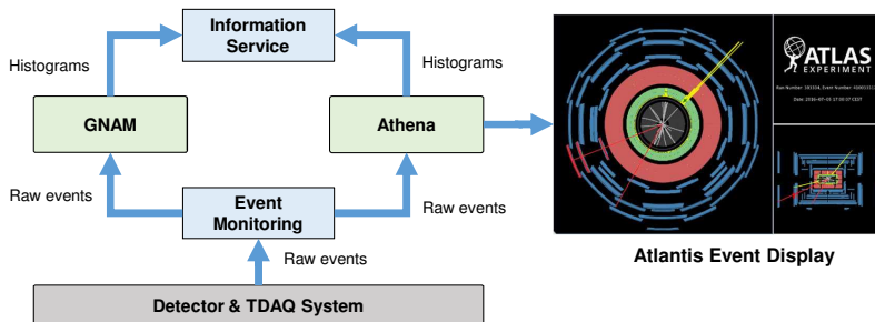
Figure 2. Event Analysis Applications interactions with the Monitoring Services.
