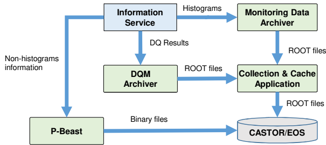
Figure 6. The Monitoring Archiving Applications interactions with the Monitoring Services.
