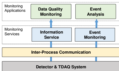
Figure 1. The high-level design of the Online Monitoring system. Shows only two Monitoring Applications as an example.
