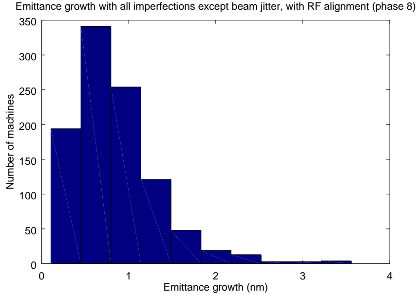
Figure 2: Distribution of the emittance growth over 1000 machines with all static imperfections implemented, after 1-2-1, DFS and RF correction, for the CLIC 380 GeV klystron-based design.
