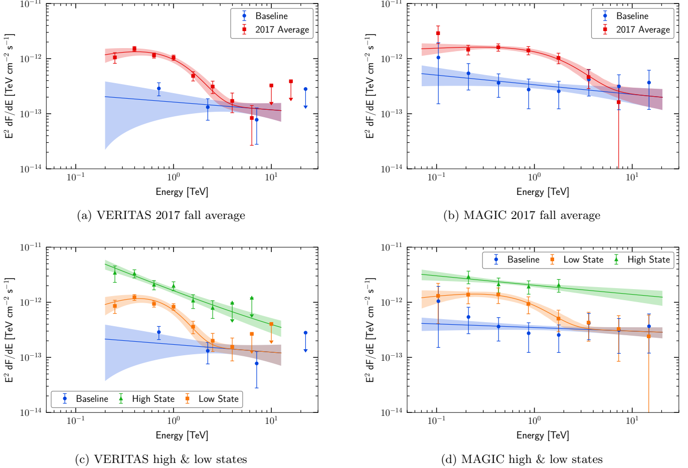
Figure 3. Spectral energy distributions for PSR J2032+4127 / MT91 213 and TeV J2032+4130 from VERITAS (left) and MAGIC (right). The blue butterflies are the spectral fits to TeV J2032+4130. The red butterflies in the upper plots are fits to the 2017 fall data: the sum of a power-law fit to TeV J2032+4130 and a cutoff power-law fit to PSR J2032+4127 / MT91 213. In the bottom plots, orange is the fit to the low-state data (PSR J2032+4127 / MT91 213 is fit with a cutoff) while green represents the high-state data (PSR J2032+4127 / MT91 213 is fit with a power law). The fit parameters are given in Table 1 and the time periods are defined in the text.
