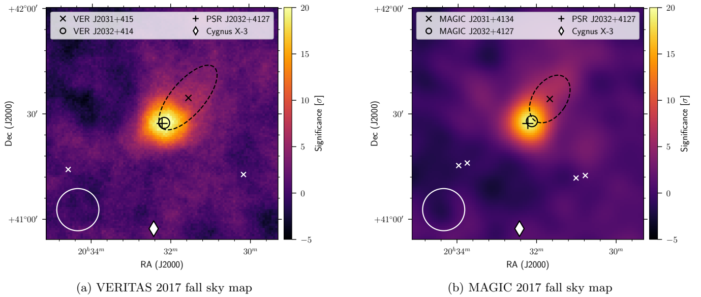
Figure 2. Significance sky maps of the region around PSR J2032+4127 / MT91 213 showing both the VERITAS (left) and MAGIC (right) results for observations during 2017 fall. The position of PSR J2032+4127 / MT91 213 is shown as a black “+”, the centroid of the gamma-ray emission as a black “o”, the position and extension for the respective telescope’s measurements of TeV J2032+4130 are shown as a black “x” and a dashed line, and the position of Cygnus X-3 is shown with a white diamond. The white circle in the lower left hand corner is of radius 0^{\circ}1 , the approximate point spread function for these measurements at 1 TeV. The wobble positions are shown as white “x”.
