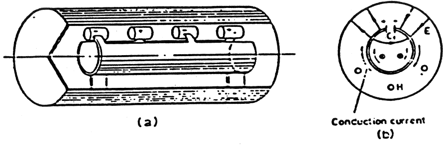
Fig. 47. The H-type structure (Teplyakov et al. (1967)). Energy range 0.5-50 MeV Effective shunt impedance at 150 MHz 600-7 MΩ/m (a) Cut-away view (not to scale). (b) Idealized cross-section in 2\pi mode.
