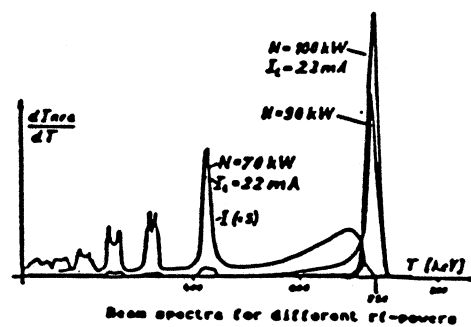
Beam spectra for different rf-powers
