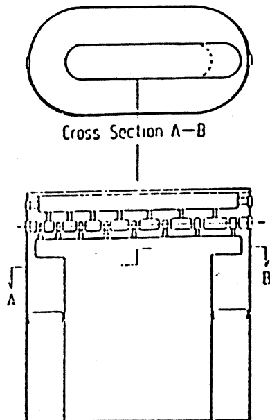
Concept of a quarter wave coaxial resonator having a race track-type cross section with drift tubes loaded at its open end.
