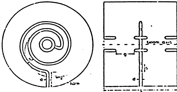
Fig. 1 Schematic drawing of a spiral resonator. Tank length L , pitch s , gap width e , tubing diameter d
