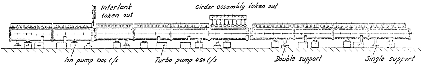
Fig. 3 Accelerating structure side view and cross-section above
