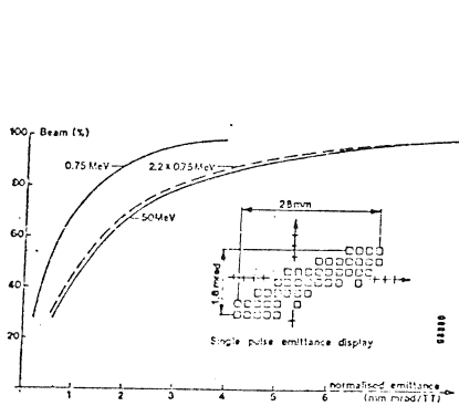
Fig. 10 Transverse emittances for I = 150 mA (H,V coincide)
