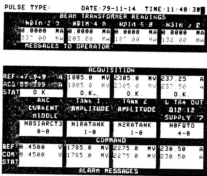
Fig. 6 Colour TV monitor on midiconsole
