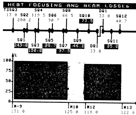
Fig. 7 Synoptic display of HEBT
