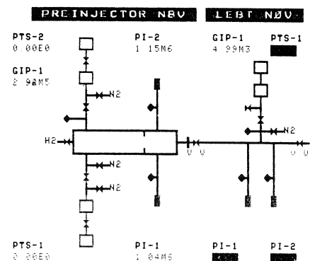
Fig. 8 Synoptic display of preinjector and LEPT vacuum
