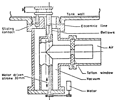
Fig. 9 RF Feed Loop (schematic)
