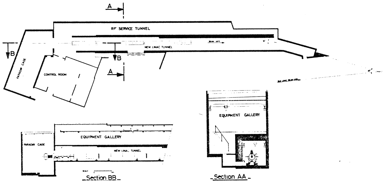
Fig. 1 New Linac Building
