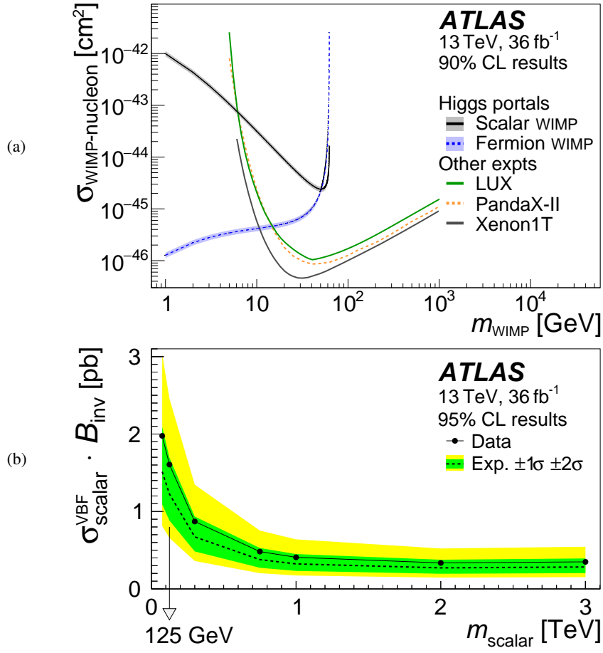
Figure 6: Upper limits on (a) the spin-independent WIMP–nucleon cross section using Higgs portal interpretations of B_{\text{inv}} at 90% CL vs. m_{\text{WIMP}} and (b) the VBF cross section times the branching fraction to invisible decays at 95% CL vs. m_{\text{scalar}} . The top plot shows results from Ref. [77–79].
