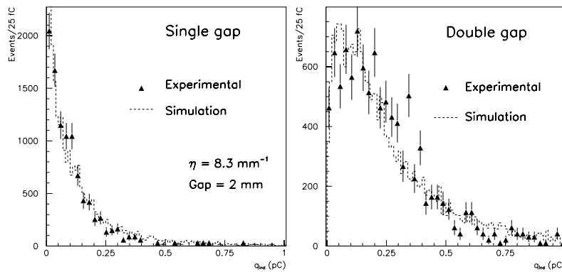
Figure 3.5: Experimental and simulated charge distributions in a single and double gap RPC.
