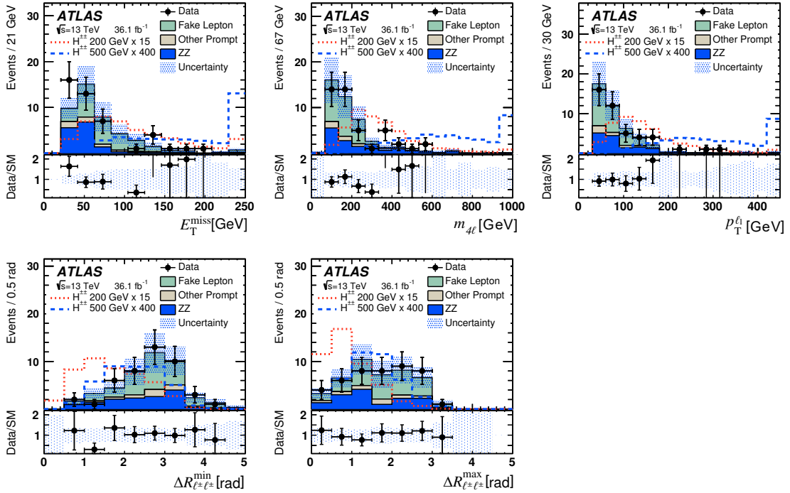
Figure 3: Distribution of variables used for the signal region optimisation of the 4\ell channel (a detailed description can be found in the caption of Figure 1).
