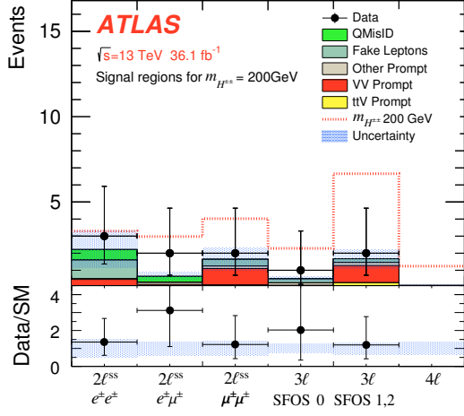
(a) 200 GeV
