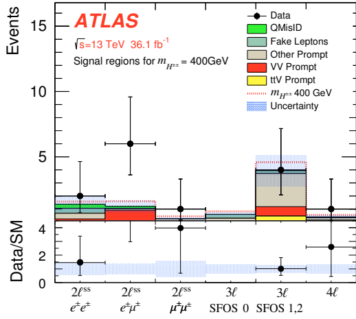
(c) 400 GeV
