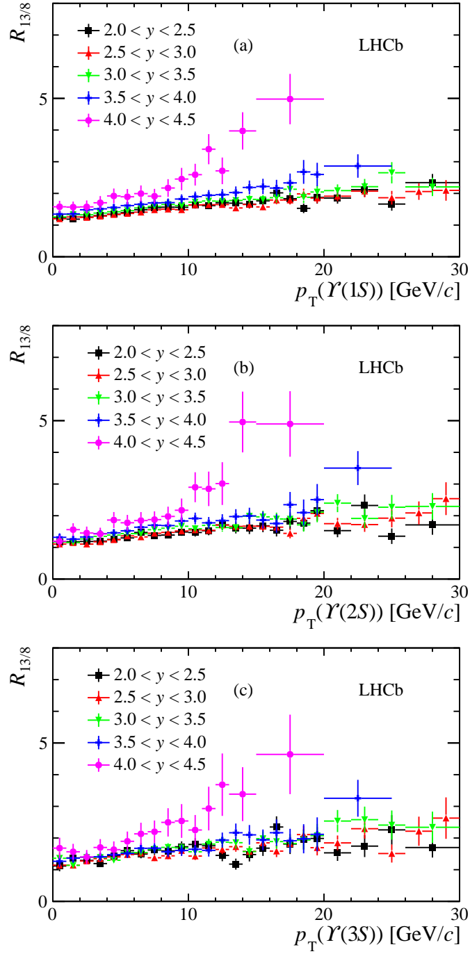
Figure 6: Ratios of double-differential cross-sections between 13 TeV and 8 TeV measurements versus p_T in intervals of y for the (a) Y(1S) , (b) Y(2S) and (c) Y(3S) states. Statistical and systematic uncertainties are added in quadrature.
