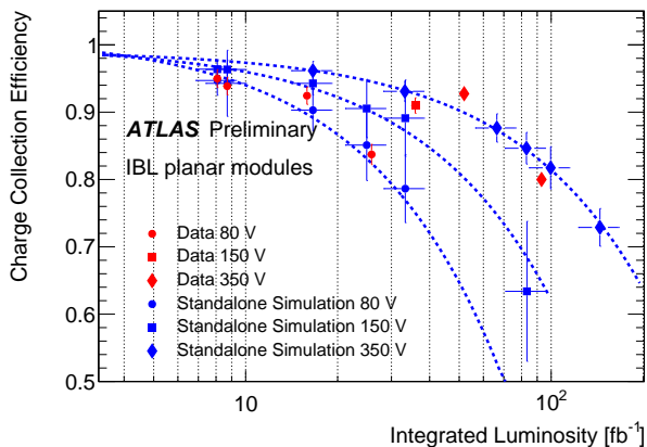
Figure 1: Charge collection efficiency as a function of luminosity. From [8]
