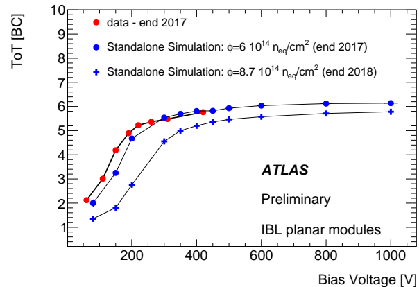
Figure 2: Most probable value of ToT as a function of bias voltage. From [8]
