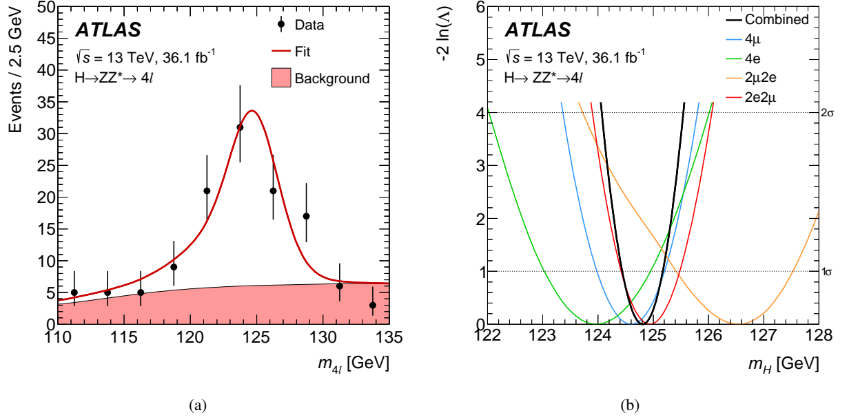
Figure 1: (a) Invariant mass distribution for the data (points with error bars) shown together with the simultaneous fit result to H \rightarrow ZZ^* \rightarrow 4\ell candidates (continuous line). The background component of the fit is also shown (filled area). The signal probability density function is evaluated per-event and averaged over the observed data. (b) Value of -2 \ln \Lambda as a function of m_H for the combined fit to all H \rightarrow ZZ^* \rightarrow 4\ell categories. The intersection of the -2 \ln \Lambda curve with the horizontal lines labelled 1\sigma and 2\sigma provide the 68.3% and 95.5% confidence intervals.
