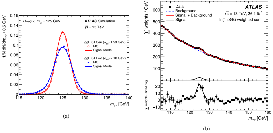
Figure 2: (a) Invariant mass distributions (circles) of simulated H \rightarrow \gamma\gamma events reconstructed in two categories with one of the best (“ggH 0J Cen”: open circles) and one of the worst (“ggH 0J Fwd”: solid circles) experimental resolutions. The signal model derived from a fit of the simulated events is superimposed (solid lines). (b) Diphoton invariant mass distribution of all selected data events, overlaid with the result of the fit (solid red line). Both for data and for the fit, each category is weighted by a factor \ln(1 + S/B) , where S and B are the fitted signal and background yields in a m_{\gamma\gamma} interval containing 90% of the expected signal. The dotted line describes the background component of the model. The bottom inset shows the difference between the sum of weights and the background component of the fitted model (dots), compared with the signal model (black line).
