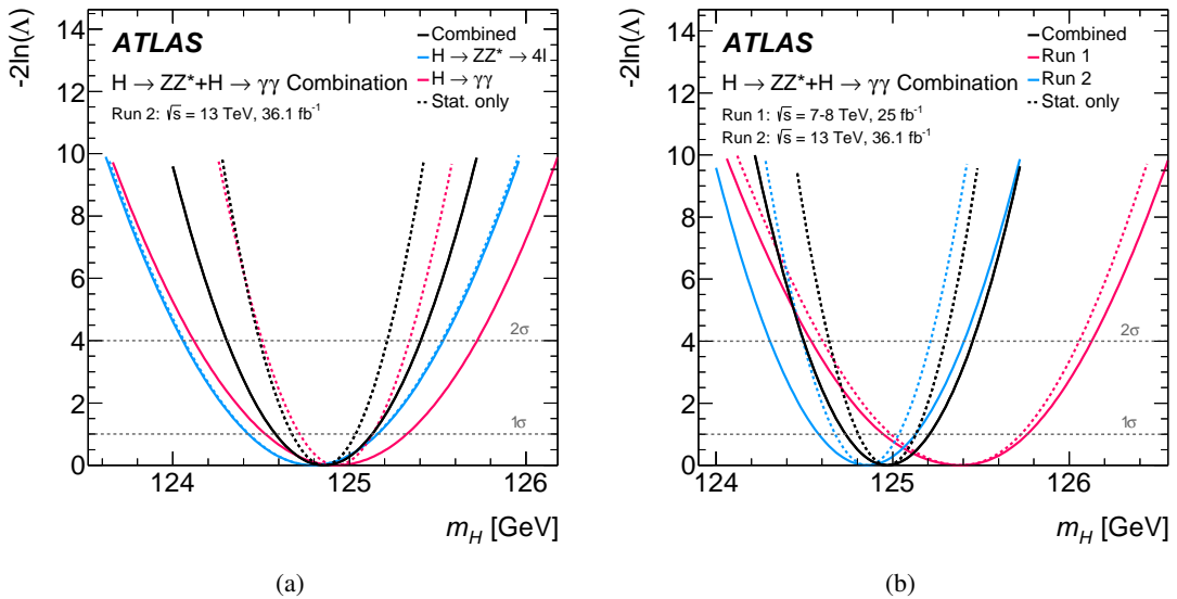
Figure 3: The value of -2 \ln \Lambda as a function of m_H for (a) H \rightarrow \gamma\gamma , H \rightarrow ZZ^* \rightarrow 4\ell channels and their combination (red, blue and black, respectively) using Run 2 data only and for (b) Run 1, Run 2 and their combination (red, blue and black, respectively). The dashed lines show the mass measurement uncertainties assuming statistical uncertainties only.
