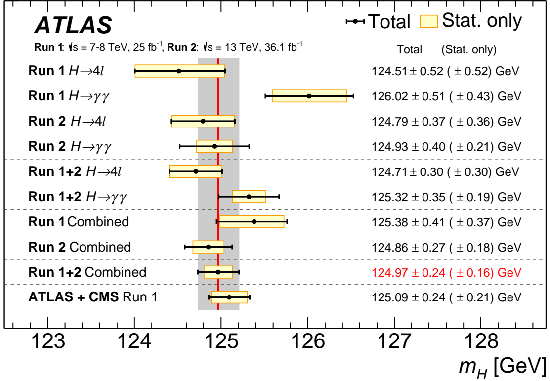
Figure 4: Summary of the Higgs boson mass measurements from the individual and combined analyses performed here, compared with the combined Run 1 measurement by ATLAS and CMS [6]. The statistical-only (horizontal yellow-shaded bands) and total (black error bars) uncertainties are indicated. The (red) vertical line and corresponding (grey) shaded column indicate the central value and the total uncertainty of the combined ATLAS Run 1 + 2 measurement, respectively.
