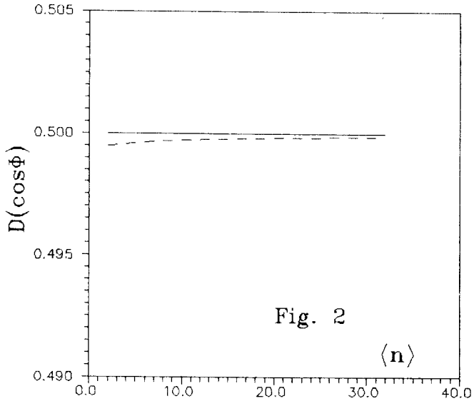
2. Dependence of the variance of the phase operator cosine upon the average occupation number for Gauss states. Solid line corresponds to the approximation (2), dashed line - to the (7) approximation.
