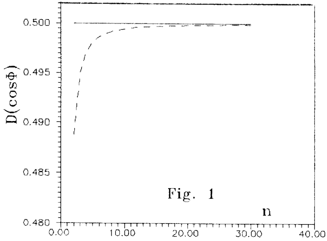
1. Dependence of the variance of the phase operator cosine upon the occupation number for the number occupation states. Solid line corresponds to the approximation (2), dashed line - to the (7) approximation.
