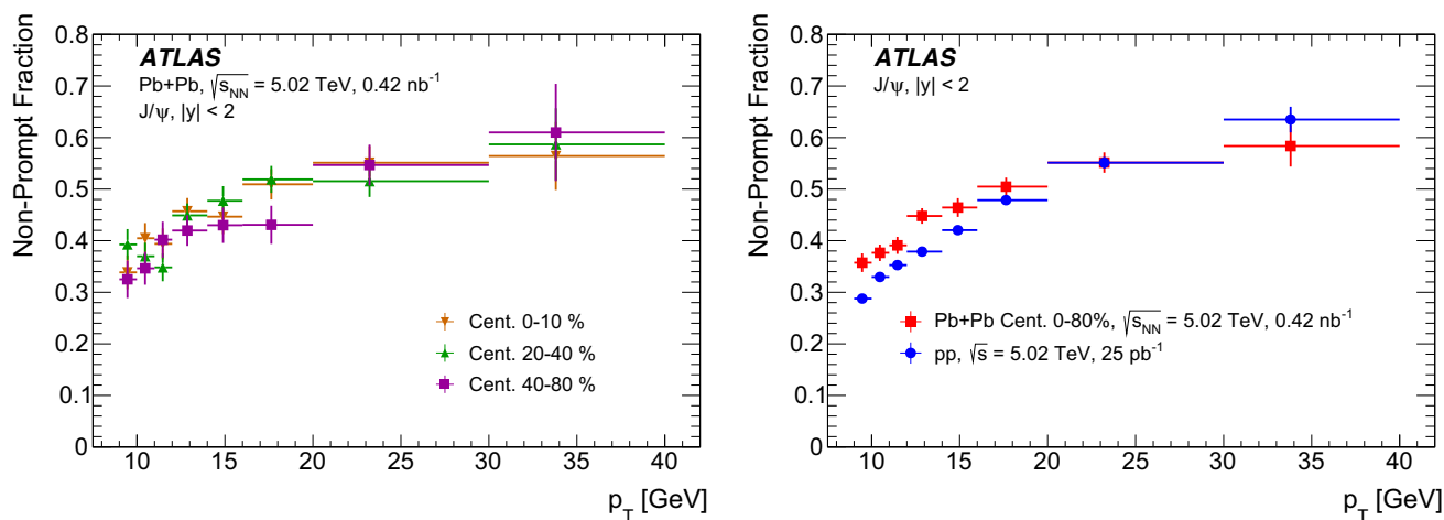
Fig. 4 (Left) Non-prompt fraction of J/\psi production in 5.02 TeV Pb+Pb collision data as a function of p_T for three different centrality slices in the rapidity range |y| < 2 . (Right) Comparison with the
