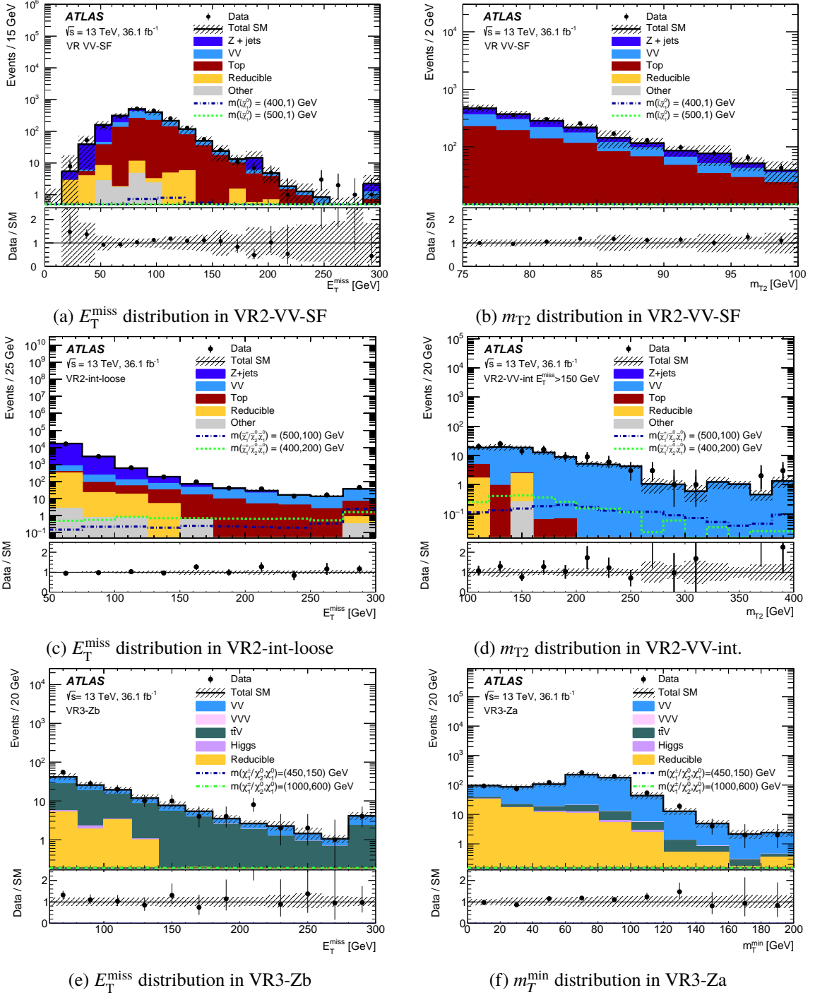
Figure 2: Distributions of E_T^{\text{miss}} , m_T^{\text{min}} , and m_{T2} for data and the estimated SM backgrounds in the (top) 2\ell+0\text{jets} channel, (middle) 2\ell+\text{jets} channel, and (bottom) 3\ell channel. Simulated signal models are overlaid for comparison. For the 2\ell+0\text{jets} ( 3\ell ) channel, the normalization factors extracted from the corresponding CRs are used to rescale the t\bar{t} and VV ( WZ ) backgrounds. For the 2\ell+0\text{jets} channel the “top” background includes t\bar{t} and Wt , the “other” backgrounds include Higgs bosons, t\bar{t}V and VVV and the “reducible” category corresponds to the data-driven matrix method estimate. For the 2\ell+\text{jets} channel, the “top” background includes t\bar{t} , Wt and t\bar{t}V , the “other” backgrounds include Higgs bosons and VVV , the “reducible” category corresponds to the data-driven matrix method estimate, and the Z+\text{jets} contribution is evaluated with the data-driven \gamma+\text{jet} template method. For the 3\ell channel, the “reducible” category corresponds to the data-driven fake-factor estimate. The uncertainty band includes all systematic and statistical sources and the final bin in each histogram also contains the events in the overflow bin.
