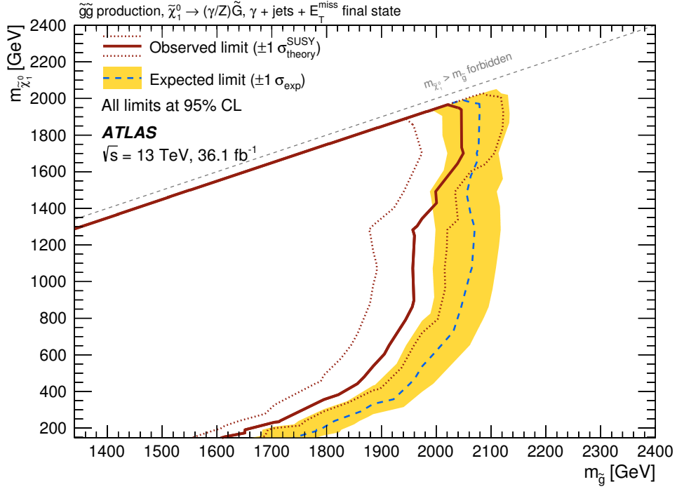
Figure 11: Derived exclusion limits for the \mu > 0 higgsino–bino GGM model explored by the photon+jets analysis. For this figure, the underlying model parameters M_3 and \mu have been transformed to the physical parameters m_{\tilde{g}} and m_{\tilde{\chi}_1^0} , subject to the assumptions stated in Section 2. For each point in the higgsino–bino parameter space, the SR ( \text{SR}_L^{\gamma j} or \text{SR}_H^{\gamma j} ) that provides the best expected sensitivity is used to estimate the exclusion likelihood. Combinations of gluino and neutralino mass are excluded at greater than 95% CL in the area to the left of the unbroken curve. The observed limits are shown for the nominal SUSY model cross-section expectation, as well as for a SUSY cross section increased and decreased by one standard deviation of the cross-section systematic uncertainty. The expected limit is also shown, along with its \pm 1 standard-deviation range.
