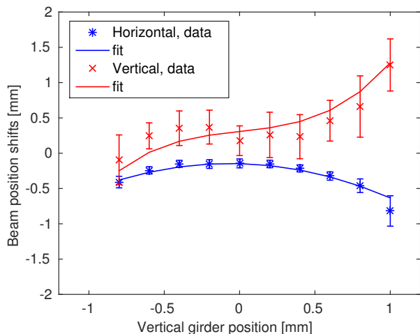
Figure 3: The measured beam position shifts for different vertical girder positions. Now we observe a third order dependence in vertical position shifts as expected. We also observe a quadratic dependence of horizontal position shifts which implies a horizontal offset.
