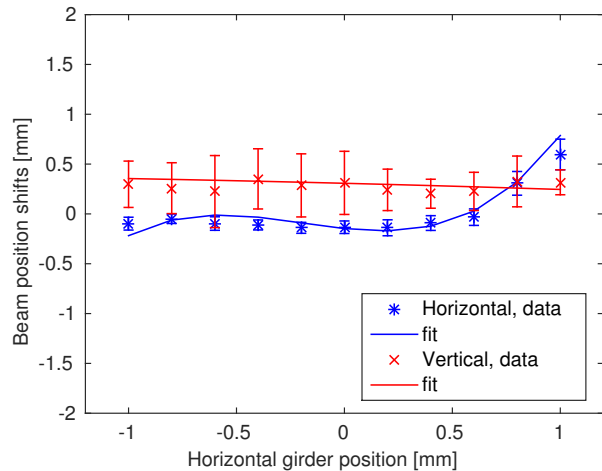
Figure 2: The measured beam position shifts for different horizontal girder positions. A third order behavior in horizontal position shifts is seen as expected.
