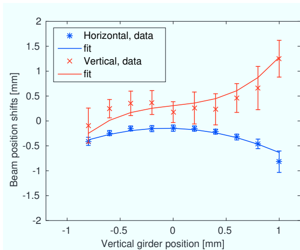
Figure 3: The measured beam position shifts for different vertical girder positions. Now we observe a third order dependence in vertical position shifts as expected. We also observe a quadratic dependence of horizontal position shifts which implies a horizontal offset.
