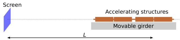
Figure 1: A schematic of the setup. Four accelerating structures are mounted on the movable girder but only the first two (the two on the right) are used. At a distance L downstream of the structure the beam position shifts can be measured with a screen.
