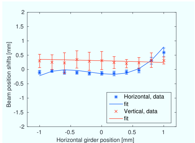
Figure 2: The measured beam position shifts for different horizontal girder positions. A third order behavior in horizontal position shifts is seen as expected.
