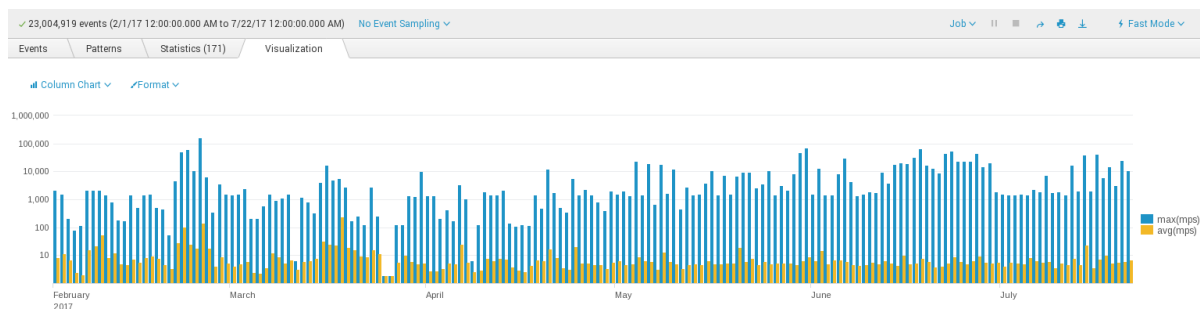
Figure 2: Maximum and average messages indexed per second, for all data indexed in course of 2017. This is a visualization of the results of a Splunk query.
