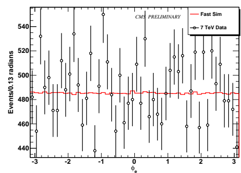
(f) Electron \phi
