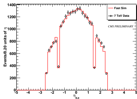
(e) Electron \eta
