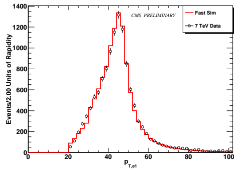
(c) Leading Electron p_T
