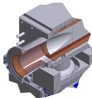
Figure 2: Detailed view of LHC collimator CAD design.
