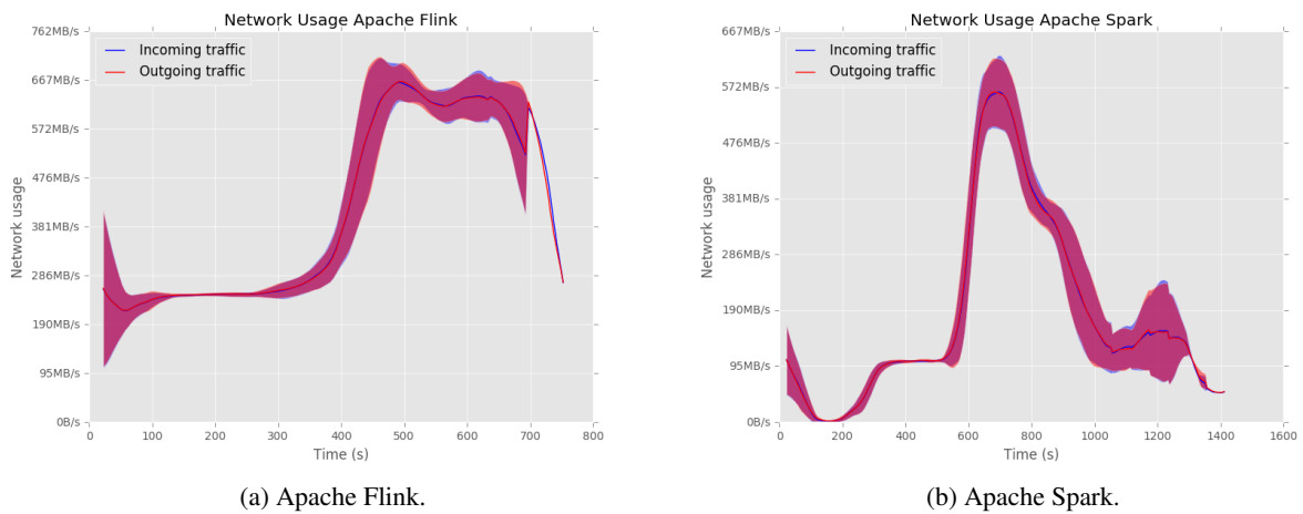
Fig. 2: Profiles of the network usage during the TeraSort job.
