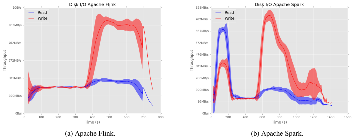
Fig. 3: Profiles of the disk usage during the TeraSort job.
