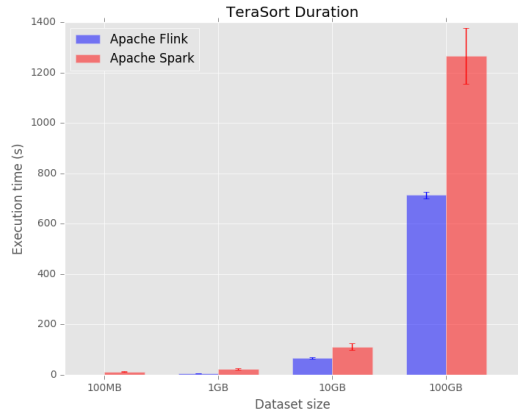
Fig. 1: The execution time of TeraSort.
