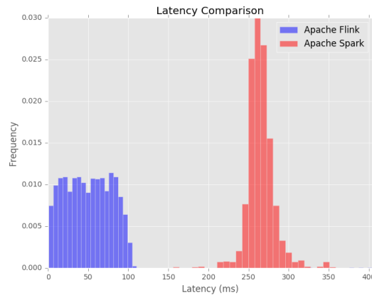
Fig. 4: The latency introduced by Apache Spark and Apache Flink.
