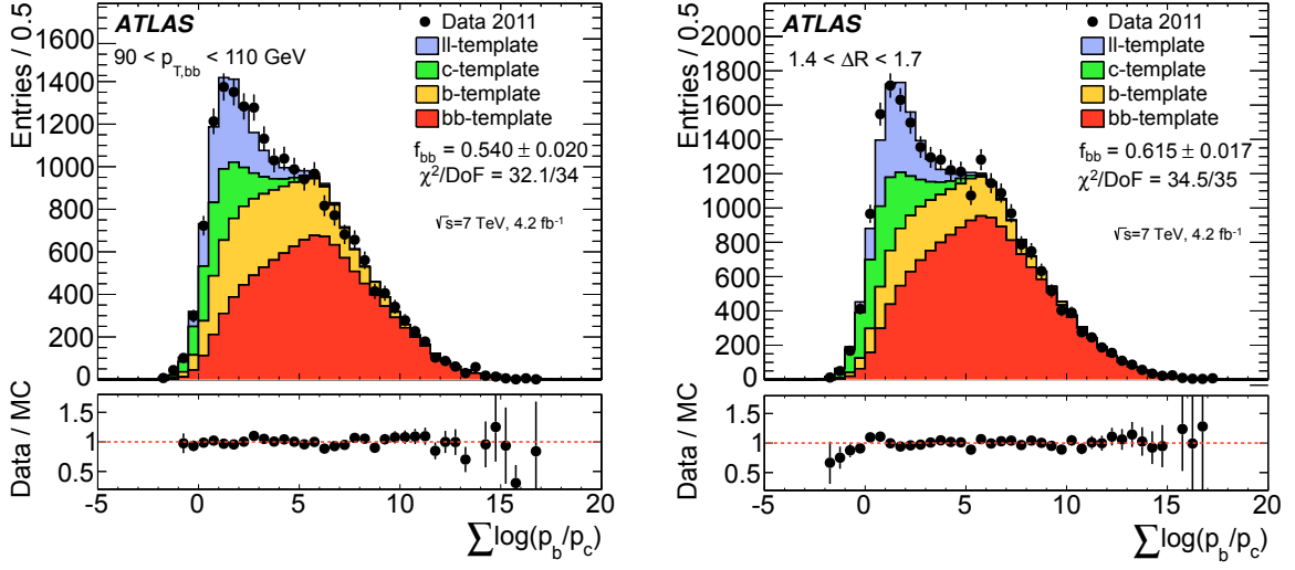
(a) 90 \text{ GeV} < p_{T,bb} < 110 \text{ GeV}
