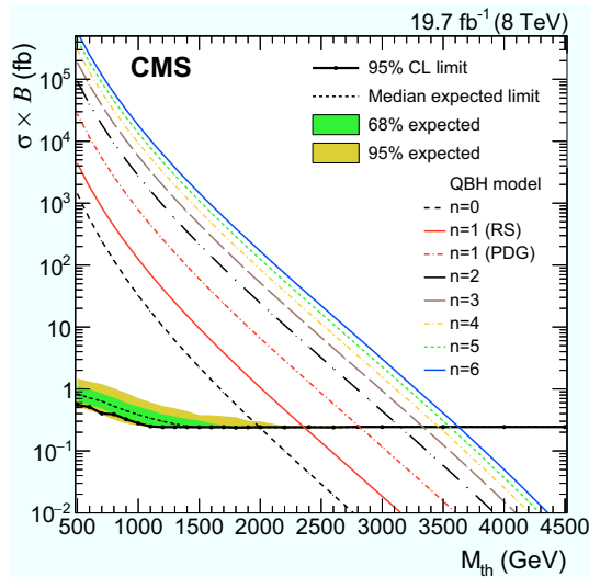
Fig. 5 The 95 % CL exclusion limit on the product of signal cross section and branching fraction for the QBH signal as a function of the threshold mass M_{th} . The limits have been calculated using the signal shape of the QBH model without extra dimensions ( n = 0 ). For signal masses M_{th} \geq 1 TeV, the change in the QBH signal shape for different numbers of extra dimensions has a negligible impact on the limit
