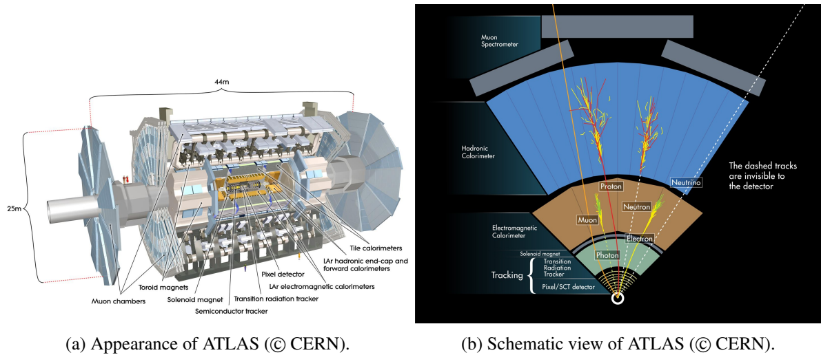
Figure 2.4: Appearance and structure of the ATLAS detector.
