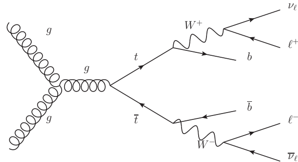
Figure 2.2: Diagram of the t\bar{t} dilepton channel.
