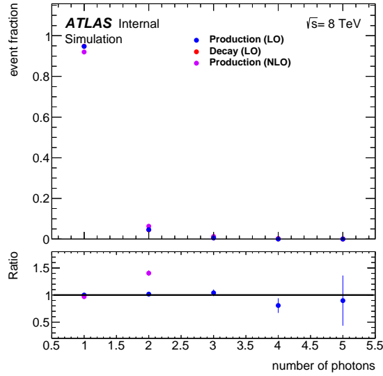
Figure 3.4: Distribution of the photon multiplicity.
