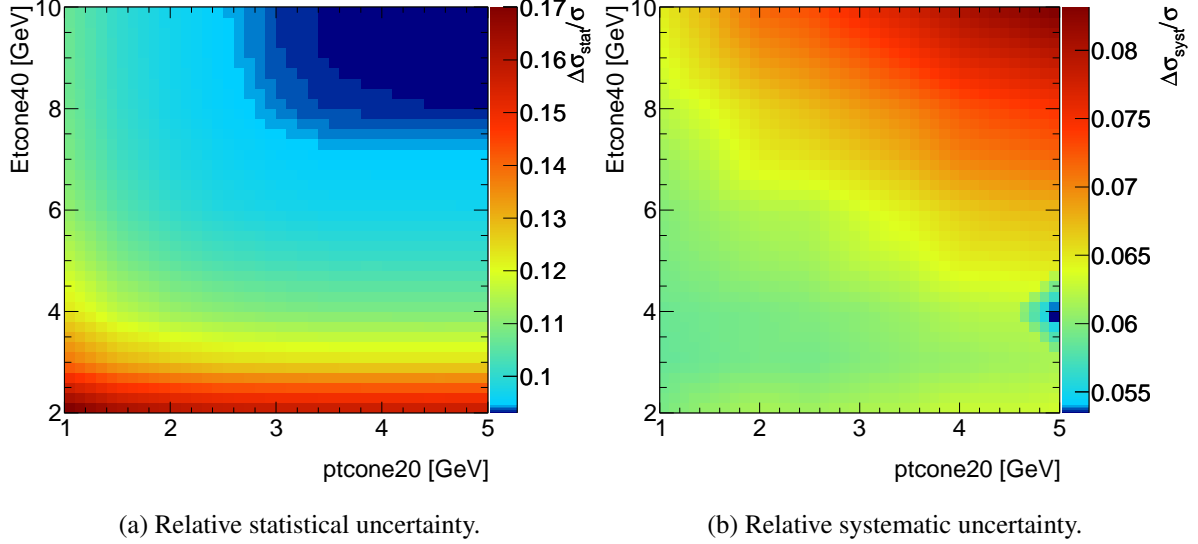
Figure 4.12: Expected relative statistical and systematic uncertainty on the cross section as a function of p_{T\text{-cone20}} and E_{T\text{-cone40}} .
