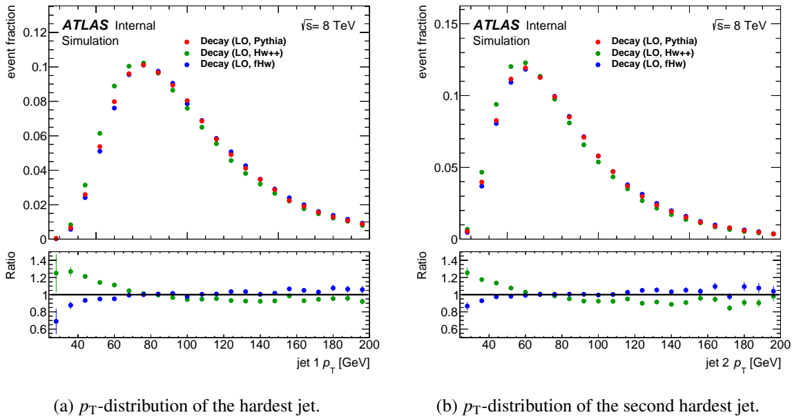
Figure 3.18: p_T distributions of the hardest jets for different parton shower generators.
