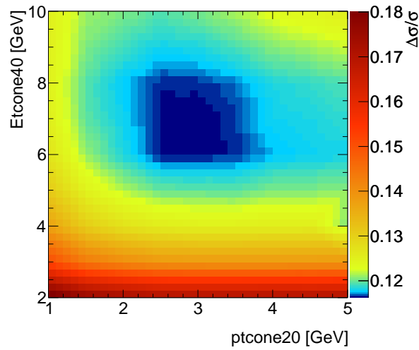
Figure 4.11: Expected relative uncertainty on the cross section \Delta\hat{\sigma} as a function of p_T -cone20 and E_T -cone40.
