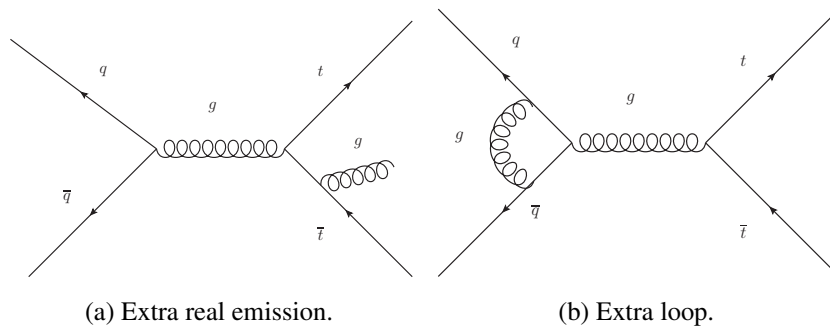
Figure 2.7: QCD NLO diagrams for the production of a t\bar{t} pair via quark annihilation.
