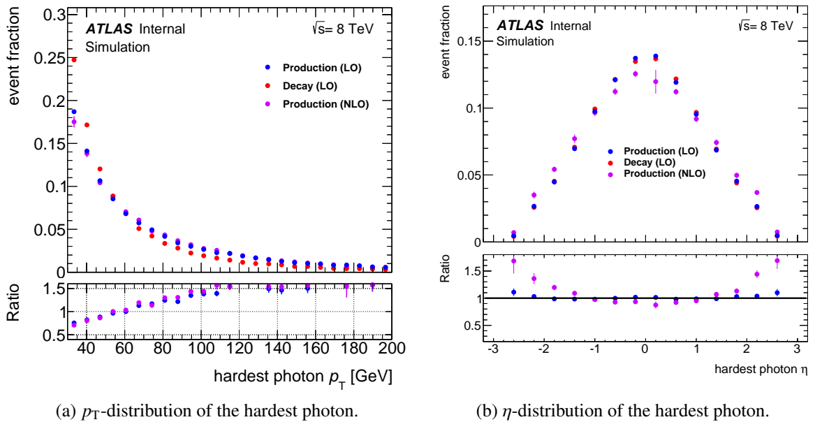
Figure 3.5: Kinematic distributions of the hardest photon.
