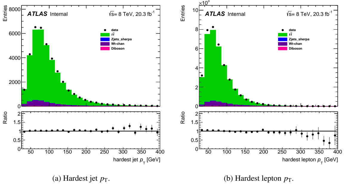
Figure 4.2: p_T distributions of the hardest jet and lepton for data compared to simulation.
