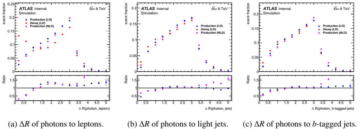
Figure 3.8: \Delta R distributions of photons to top decay products.
