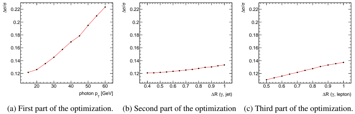
Figure 4.9: Comparison of the results for the photon's p_T , the \Delta R of the photon and any jet and the \Delta R of the photon and any lepton.
