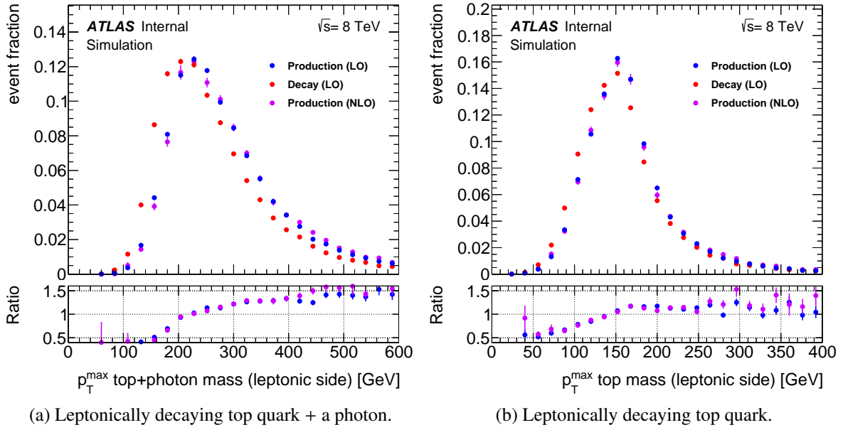
Figure 3.16: Invariant mass distributions of the leptonically decaying top with the p_T^{\max} method.
