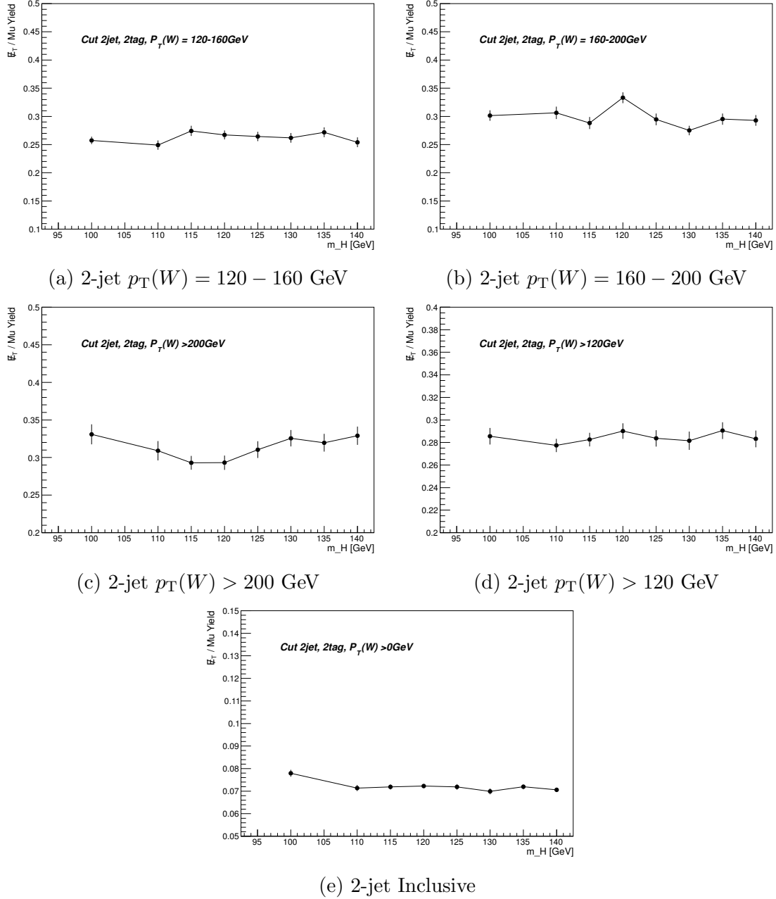
Figure A.1: Ratio of exclusive E_T^{\text{miss}} triggered to muon triggered signal yields in the different cut-based 2-jet, 2-tag signal regions as a function of Higgs mass, m_H . The yields are all profit Monte Carlo expectations. The different b-tagging regions (LL,MM,TT) are merged as no significant difference is observed between these regions. The error on each point contains only statistical and trigger uncertainties.
