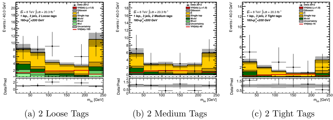
Figure 7.9: Prefit distributions of dijet invariant mass, m_{bb} , in the cut-based E_T^{\text{miss}} triggered 3-jet p_T(W) = 160 - 200 GeV region. Format is the same as Figure 7.5.
