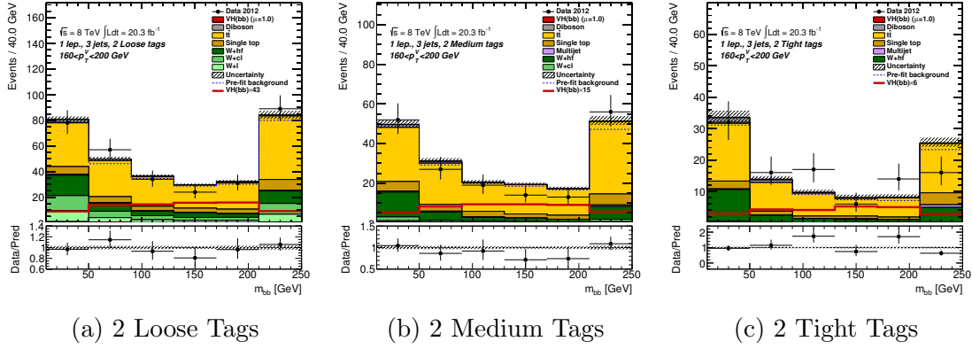
Figure D.9: Positfit distributions of dijet invariant mass, m_{bb} , in the cut-based combined 3-jet p_T(W) = 160 - 200 GeV regions. The format is the same as Figure D.1.
