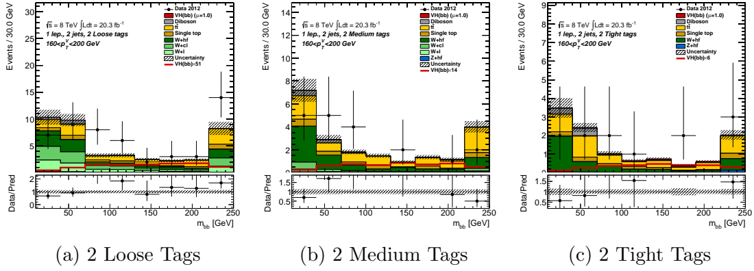
Figure 7.6: Prefit distributions of di-b-jet invariant mass, m_{bb} , in the cut-based E_T^{\text{miss}} triggered 2-jet p_T(W) = 160 - 200 GeV region. Format is the same as Figure 7.5.
