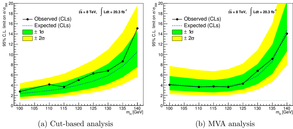
Figure 10.11: Expected and observed limits from the 95% CL upper bound on the cross section times branching ratio as a function of m_H for the E_T^{\text{miss}} triggered analyses. Values are expressed as a multiple of the standard model expectation. The observed values are shown as a solid line while the expected values, for the background-only case, are shown as a dashed line with the green and yellow shaded areas representing the \pm 1\sigma and \pm 2\sigma shifts from the central expected value. The grey dashed line represents the Standard Model value of \hat{\mu} = 1.0 .
