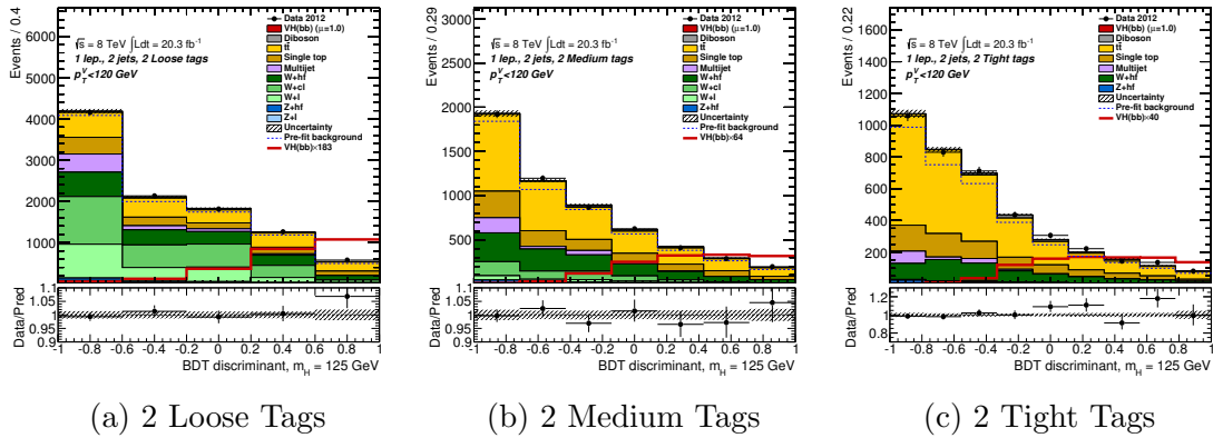
Figure D.12: Postfit distributions of the BDT output in the MVA combined 2-jet p_T(W) < 120 \text{ GeV} regions. The format is the same as Figure D.1.
