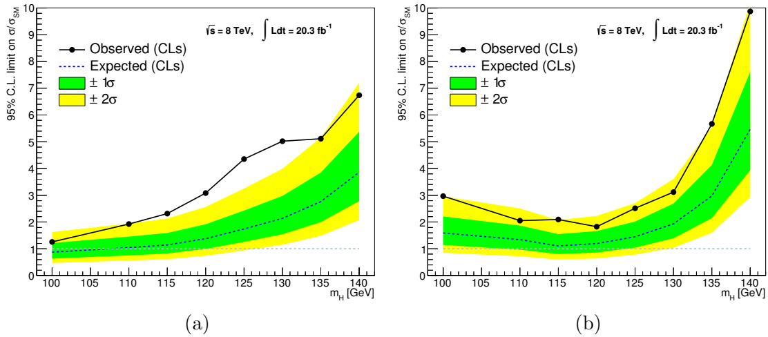
Figure C.1: Expected and observed limits from the 95% CL upper bound on the cross section times branching ratio as a function of m_H for the nominal analyses. Values are expressed as a multiple of the standard model expectation. The observed is shown as a solid line while the expected, for the background only case, is shown as a dashed line with the green and yellow shaded areas representing the \pm 1\sigma and \pm 2\sigma shifts from the expected.
