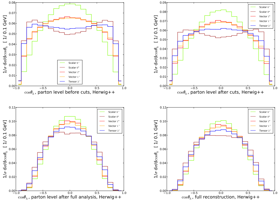
Figure 6.7.: Cosine of the helicity angle \theta_h , Eq. 1.17c, calculated from the hadronically decaying Z at different steps of the analysis: Inclusive Monte Carlo generation level (top, left), Monte Carlo generation level including selection cuts Eqs. 6.7-6.8 (top, right), after the full subjet analysis including Monte Carlo truth information (bottom, left), and after the full analysis (bottom, right).
