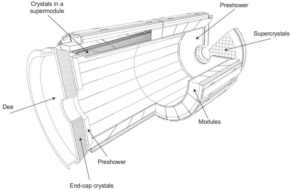
Figure 2.6.: Overview of the electromagnetic calorimeter.
