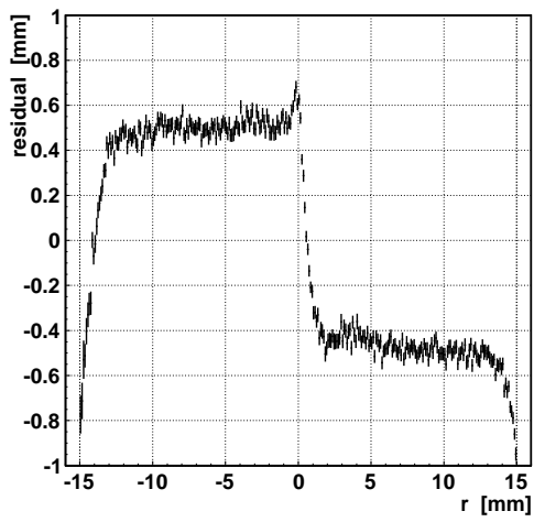
Figure 4.7: z -shift: left: Residual for negative slopes; right: Residual for positive slopes.
