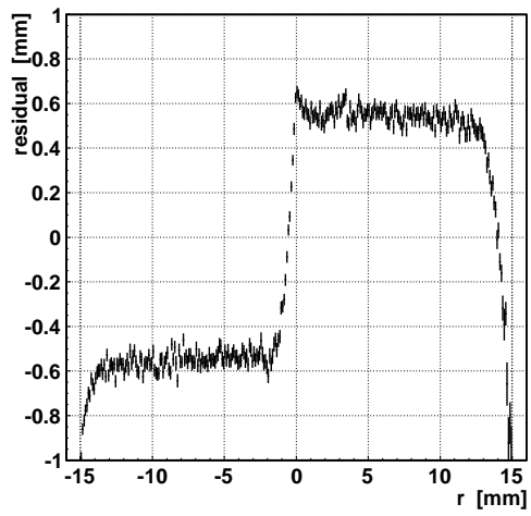
Figure 4.7: z -shift: left: Residual for negative slopes; right: Residual for positive slopes.
