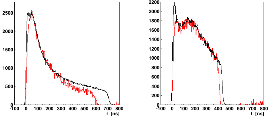
Figure 5.15: Drift time spectra measured in the GIF. The left plot shows the spectra in case of Ar:CO 2 93:7 without irradiation (black) and at an irradiation level of 1900 \frac{\text{Hz}}{\text{cm}^2} (red). On the right plot the situation for the alternative gas mixture Ar:CO 2 :N 2 96:3:1 is shown without (black) and with \gamma -irradiation (red).
