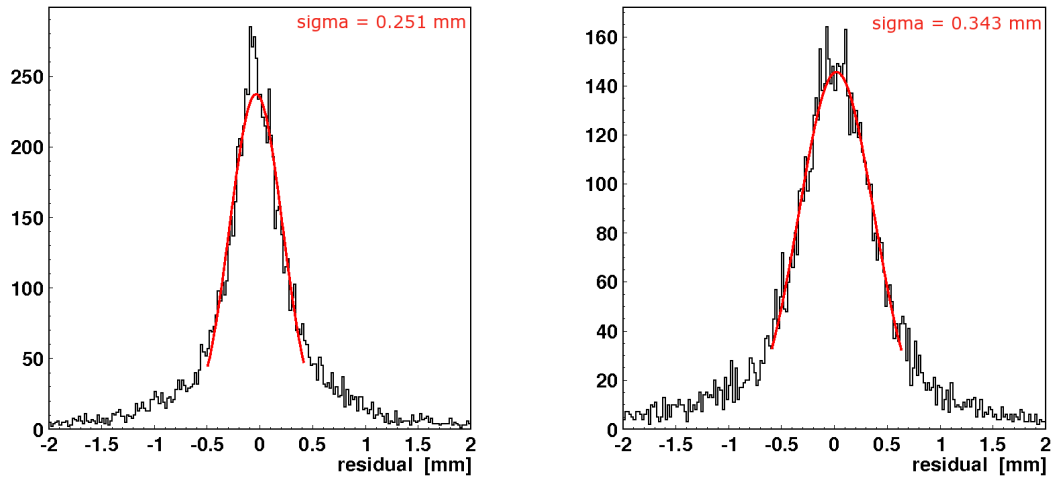
Figure 5.18: Width of residual in case of no \gamma -background (left) and with background (right).
