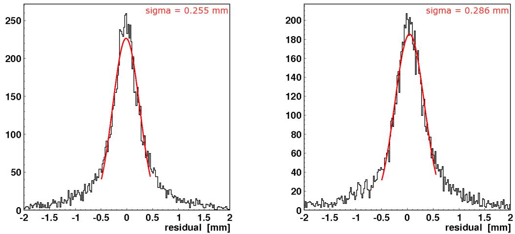
Figure 5.19: Width of residual in case of no \gamma -background (left) and with background (right).
