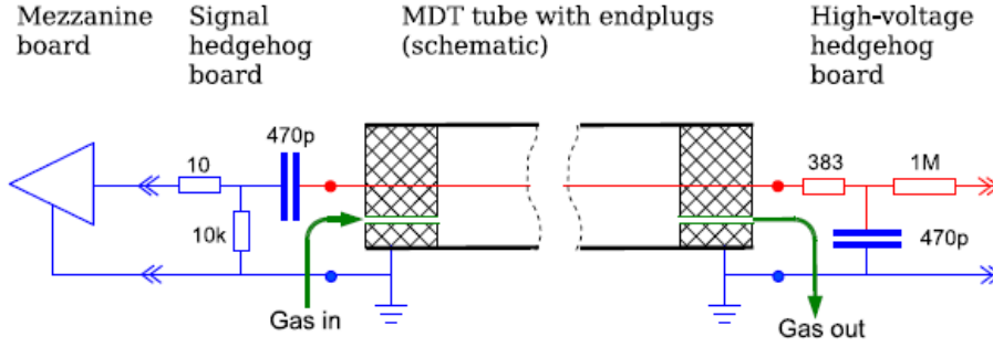
Figure 2.3: Service connections to a MDT tube. [20]
