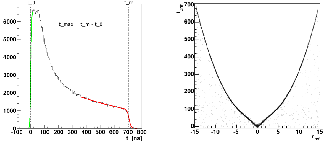
Figure 4.1: left: Drift time spectrum; right: rt -relation.
