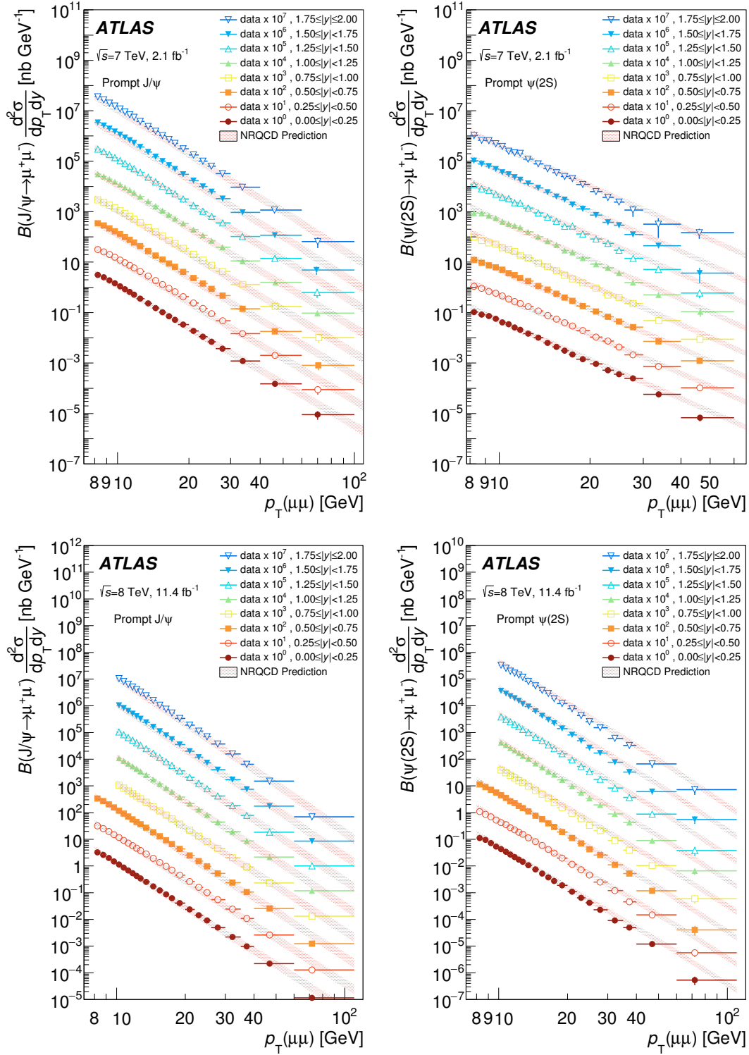
Figure 7: The differential prompt cross-section times dimuon branching fraction of J/\psi (left) and \psi(2S) (right) as a function of p_T ( \mu\mu ) for each slice of rapidity. The top (bottom) row shows the 7 TeV (8 TeV) results. For each increasing rapidity slice, an additional scaling factor of 10 is applied to the plotted points for visual clarity. The centre of each bin on the horizontal axis represents the mean of the weighted p_T distribution. The horizontal error bars represent the range of p_T for the bin, and the vertical error bar covers the statistical and systematic uncertainty (with the same multiplicative scaling applied). The NLO NRQCD theory predictions are also shown.
