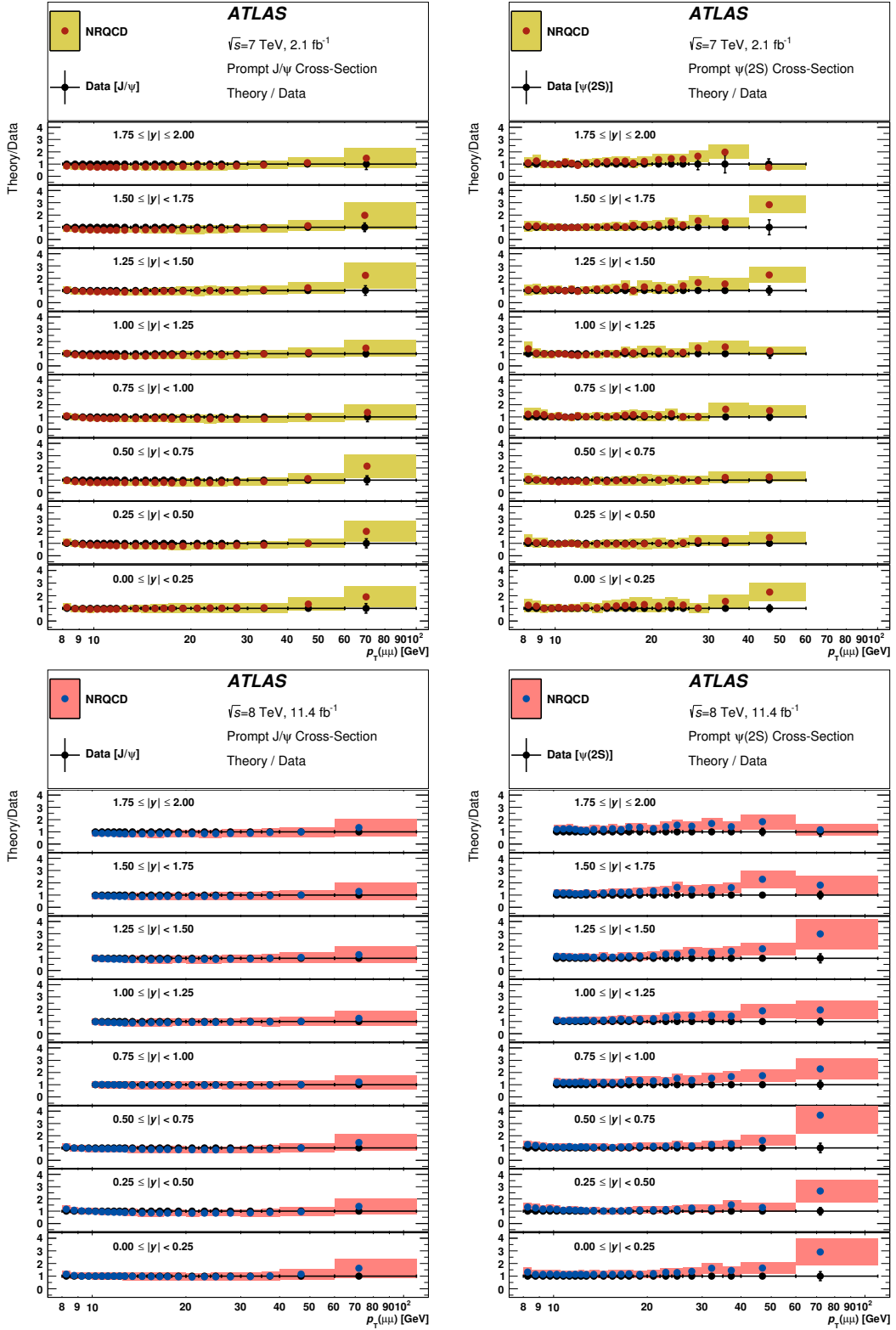
Figure 11: The ratios of the NRQCD theoretical predictions to data are presented for the differential prompt cross-section of J/\psi (left) and \psi(2S) (right) as a function of p_{T,(\mu\mu)} for each rapidity slice. The top (bottom) row shows the 7 TeV (8 TeV) results. The error on the data is the relative error of each data point, while the error bars on the theory prediction are the relative error of each theory point.
