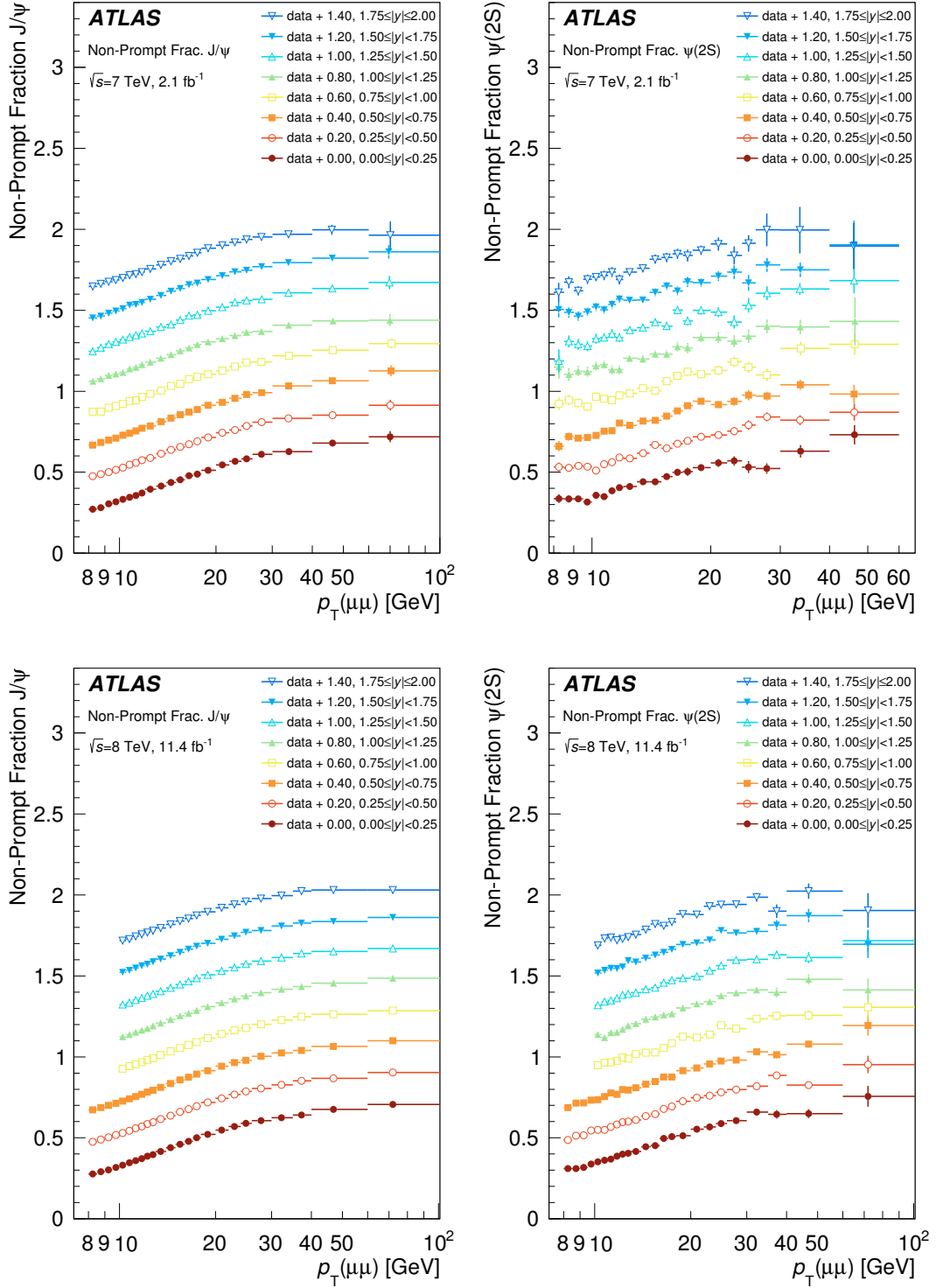
Figure 9: The non-prompt fraction of J/\psi (left) and \psi(2S) (right), as a function of p_T ( \mu\mu ) for each slice of rapidity. The top (bottom) row shows the 7 TeV (8 TeV) results. For each increasing rapidity slice, an additional factor of 0.2 is applied to the plotted points for visual clarity. The centre of each bin on the horizontal axis represents the mean of the weighted p_T distribution. The horizontal error bars represent the range of p_T for the bin, and the vertical error bar covers the statistical and systematic uncertainty (with the same multiplicative scaling applied).
