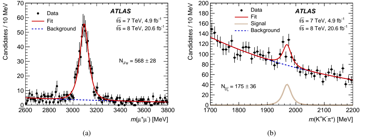
Figure 4: Mass distribution of the (a) J/\psi and (b) D_s^+ candidates after the full B_c^+ \rightarrow J/\psi D_s^{*\pm} selection (without mass constraints in the cascade fit) in the mass window of the B_c^+ candidate 5900 \text{ MeV} < m(J/\psi D_s^+) < 6400 \text{ MeV} . The spectra are fitted with a sum of an exponential and a modified Gaussian function. The uncertainties of the shown J/\psi and D_s^+ yields are statistical only.
