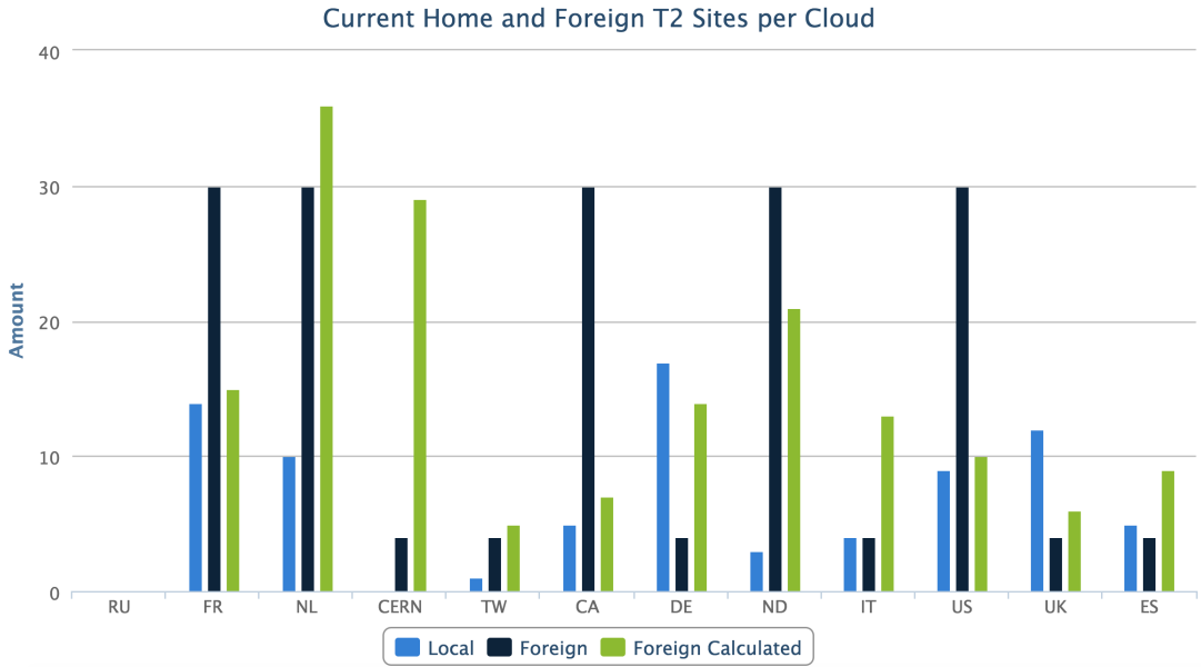
Figure 11. Dynamic cloud potential
