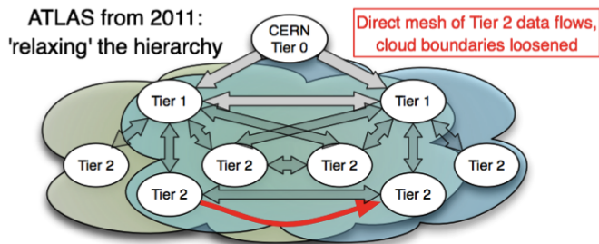
Figure 10. Data flows in mesh model
