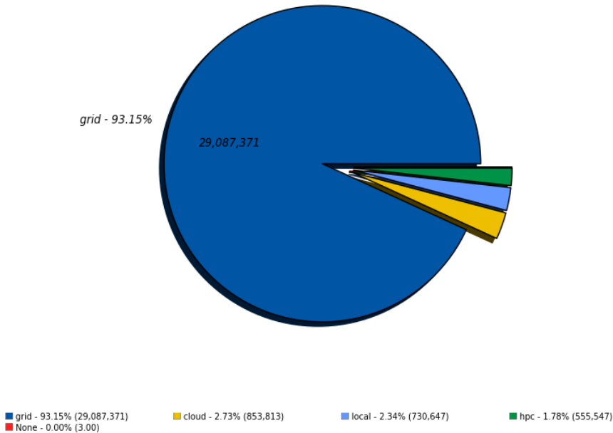
Figure 4. Jobs by resource type. Period 6 June to 5 July 2015.
