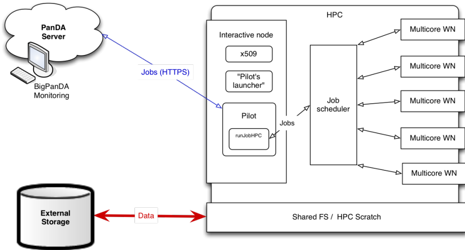
Figure 6. HPC integration in PanDA
