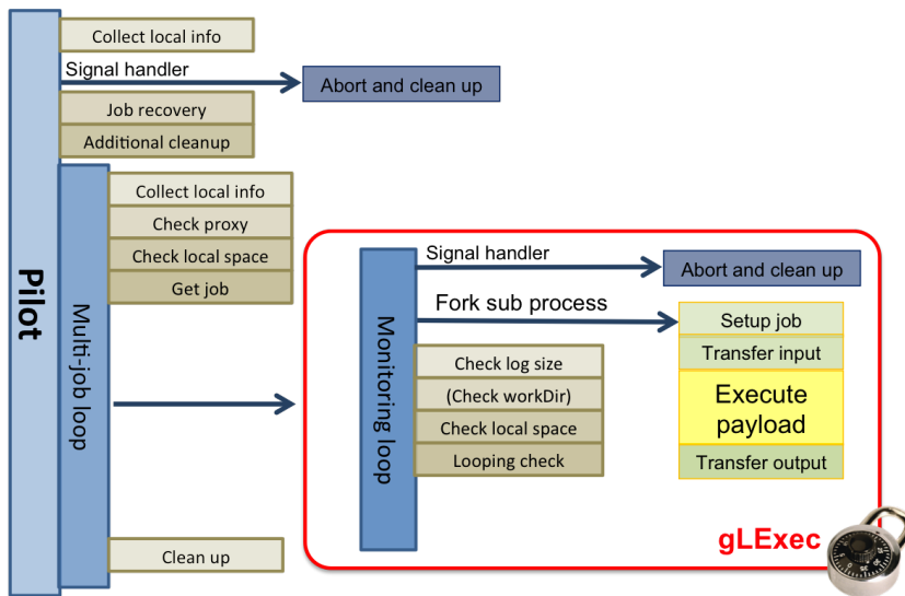
Figure 2. High level diagram of the PanDA Pilot
