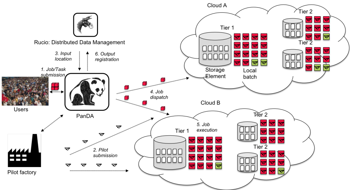
Figure 1. High level diagram of the PanDA system
