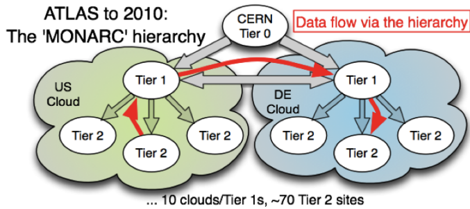
Figure 9. Data flows based on MONARC model
