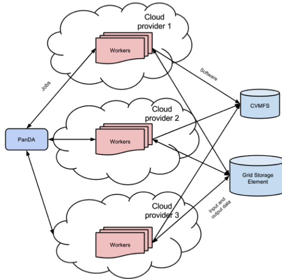
Figure 5. Cloud Computing integration schema
