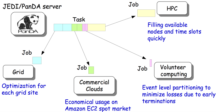
Figure 8. JEDI dynamic job definition
