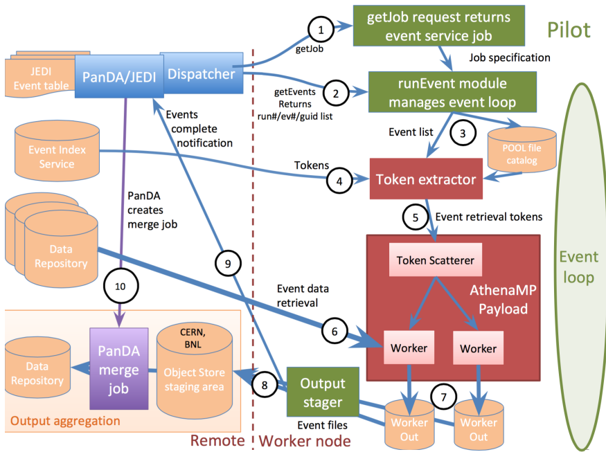
Figure 7. Event Service Schematic
