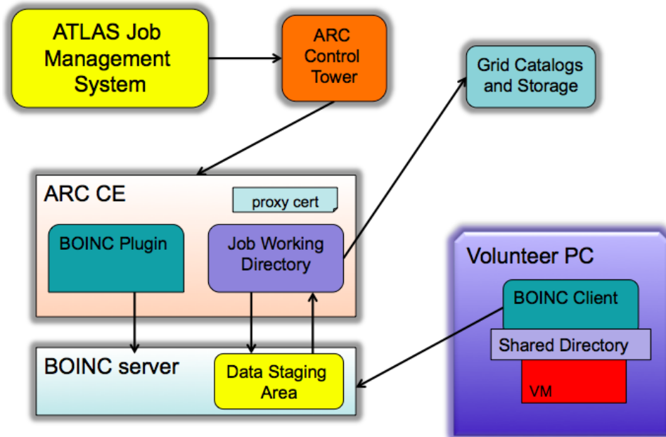
Figure 1. Architecture of ATLAS@Home.
