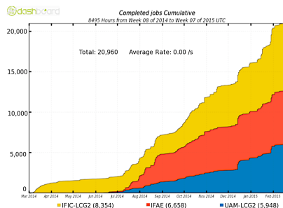
Figure 5(a). Completed multicore jobs in the ES-ATLAS-T2 sites since March 2014.
