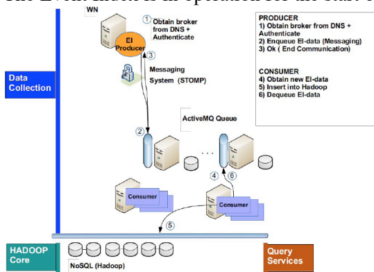
Figure 8. Event Index architecture
