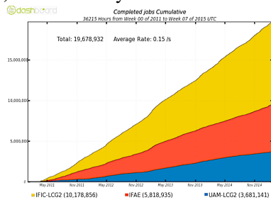
Figure 3(a). Completed jobs (50% analysis, 50% production) in the ES-ATLAS-T2 sites during Run 1 and before Run 2.
