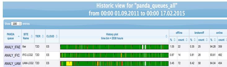
Figure 2. ATLAS availability for the ES-ATLAS-T2 analysis queues.
