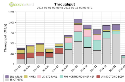
Figure 6. Aggregated XRootD Traffic at various Tiers of ATLAS.
