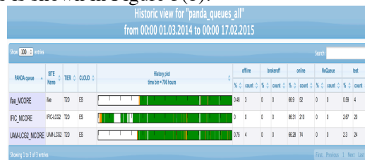
Figure 5(b). ATLAS availability for the ES-ATLAS-T2 multicore queues since March 2014.
