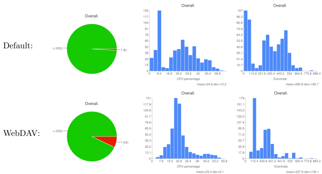
Figure 4. Overall performance of the fast analysis at all sites for the default PanDA access (top) and the WebDAV access (bottom). Shown are the fraction of successful and failed jobs (left), the CPU utilisation fraction (middle) and the event rate (right).
