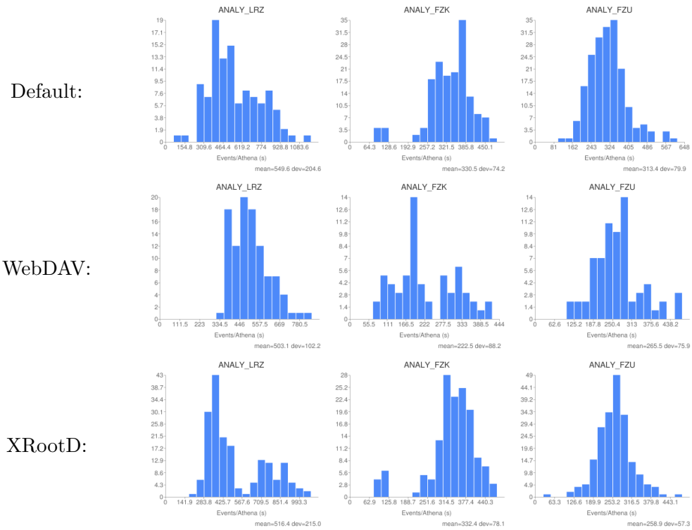
Figure 5. The event rate for the fast analysis for LRZ-LMU (left), FZK (middle) and Prague/FZU (right). Shown are the default PanDA access modes (top), WebDAV (middle) and XRootD (bottom).
