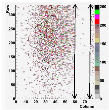
Figure 2. Latch upset map.
