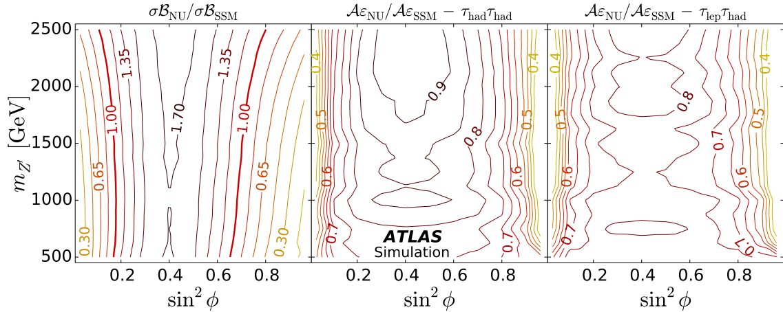
Figure 5. Signal production cross section times \tau^+\tau^- branching fraction for Z'_{NU} , \sigma\mathcal{B}_{NU} , divided by \sigma\mathcal{B}_{SSM} (left) and acceptance times efficiency for Z'_{NU} , \mathcal{A}\varepsilon_{NU} , divided by \mathcal{A}\varepsilon_{SSM} for the (middle) \tau_{had}\tau_{had} and (right) \tau_{lep}\tau_{had} channels, as a function of \sin^2 \phi and m_{Z'} .
